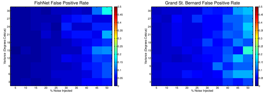
Fig. 18. False Positive rates as a function of both noise variance (Y-axis) and percentage of data points modified by noise (X-axis). The shade of color associated with each grid cell reflects the degree of precision (on a scale of 0% to 50%) for that configuration of noise level and saturation.
