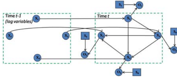
Fig. 7. Time slices are designated by the dashed rectangles. The variables within the dashed area an abstract representation of the learned spatial model among four sensor variables. A sensor state variable and an observation variable are attached to each of the four sensor variables in the current time slice.
