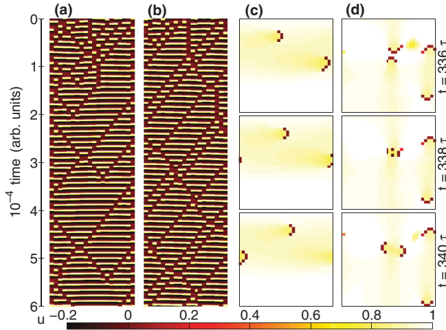
FIG. 4. (Color online) (a), (b) Spatio-temporal evolution of a system of coupled relaxation oscillators showing traveling waves of phase defects in (a) a linear array with passive elements at the boundaries and (b) with periodic boundary conditions. (c), (d) Propagating defects in two-dimensional media with periodic boundary condition showing (c) two horizontally moving “gliders” and (d) collision of two “gliders.” For clear visualization of the motion of the spatially extended defects, snapshots of the two-dimensional medium are taken at intervals which are multiples of the oscillation period for the mean activity of the system \tau .
