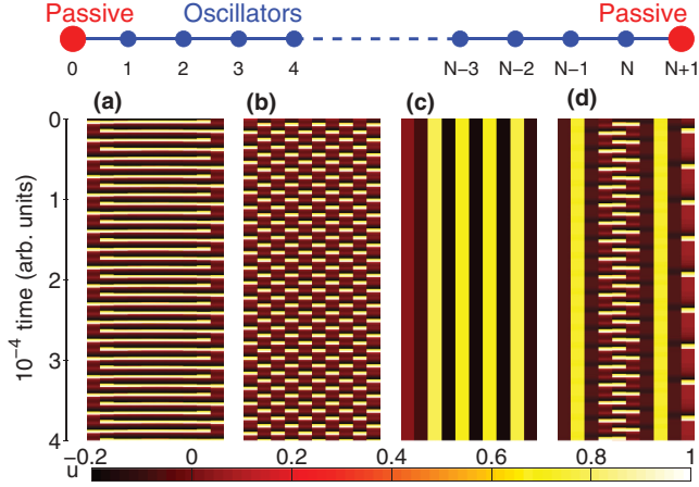
FIG. 1. (Color online) Spatiotemporal evolution of a one-dimensional array of coupled relaxation oscillators ( N = 10 ) with passive elements at the boundaries (model system shown schematically on top). Pseudocolor plots of the activation variable u indicate different regimes characterized by (a) synchronized oscillations (SO), (b) antiphase synchronization (APS), (c) spatially patterned oscillator death (SPOD), and (d) chimera state (CS), i.e., co-occurrence of spatial patches with dynamically distinct behavior.
