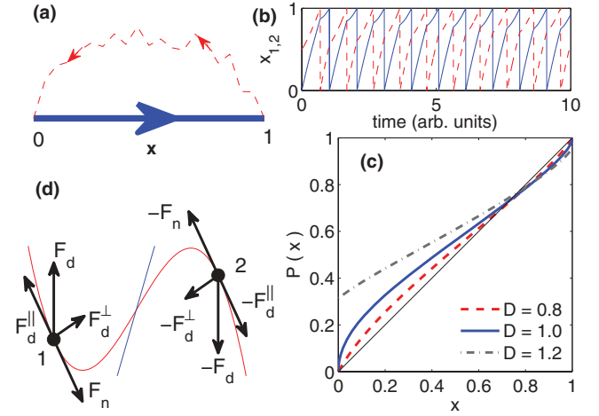
FIG. 3. (Color online) (a) Schematic diagram of a limit cycle trajectory for an oscillator in the relaxation limit ( \epsilon \rightarrow 0 ) and extreme asymmetry (for details see text), such that the oscillator is on the solid line ( 0 < x < 1 ) for its entire period. (b) Time series of two such coupled oscillators [Eq. (3) with D = 1 ] and (c) the Poincaré map for the system at different coupling strengths D showing stable antiphase synchronization. (d) Phase-plane diagram indicating the general mechanism (see text) for oscillator death in a system of two coupled oscillators (1 and 2).
