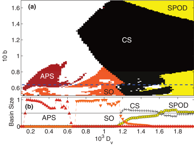
FIG. 2. (Color online) Different dynamical regimes of a one-dimensional array of coupled relaxation oscillators ( N = 10 ) in the D_v - b parameter plane, showing regions where the majority ( >50\% ) of initial conditions result in synchronized oscillations (SO), antiphase synchronization (APS), spatially patterned oscillator death (SPOD), and chimera state (CS). (b) Variation of the attraction basin size for the different regimes mentioned above (measured as fraction of initial states reaching the attractor), with coupling strength D for b = 0.064 [i.e., along the broken line shown in panel (a)]. In practice, the regimes are distinguished by thresholds applied on the order parameters \langle \sigma_i^2(u_i) \rangle , \langle \sigma_i^2(u) \rangle_t , \langle \sigma_{\text{even}}^2(u) \rangle_t and \langle \sigma_{\text{odd}}^2(u) \rangle_t , which have been taken to be 0.05 for the present figure. Basin sizes have been estimated using 10^4 initial conditions.
