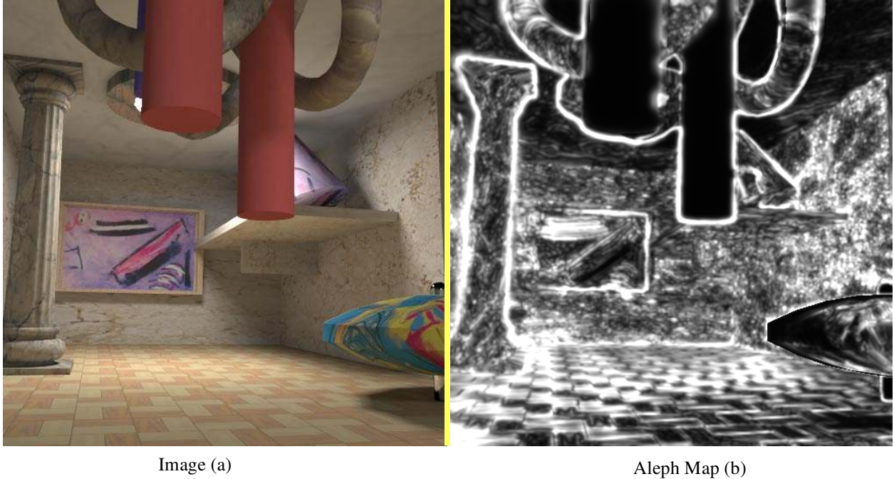
Figure 10: Spatiotemporal sensitivity visualization ( see color plate ). Image (a) and its corresponding error tolerance map, the Aleph Map (b). Note that the spinning top in the bottom right has reduced tolerance to error although it has textures and is moving. This is due to the information introduced by the saliency map, telling the algorithm to be stricter on the top because the viewer will more likely focus attention there. The red beams are treated strictly because there are no high frequency details.
