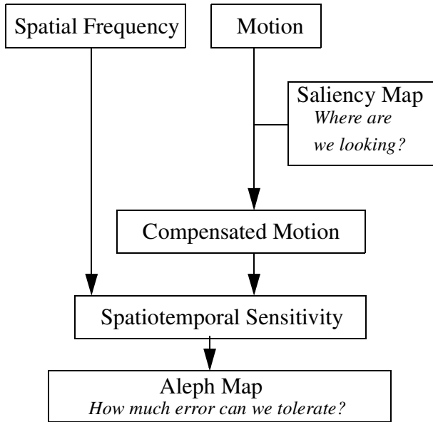
Figure 2: Flowchart outlining the computation of spatiotemporal error tolerance. The Aleph Map is a perceptual oracle derived from the spatial frequency, motion and visually important information in a scene. The saliency map is a measure of visual attention and is used to compensate for eye tracking movements in order to fully take advantage of perceptual sensitivity in dynamic scenes.
