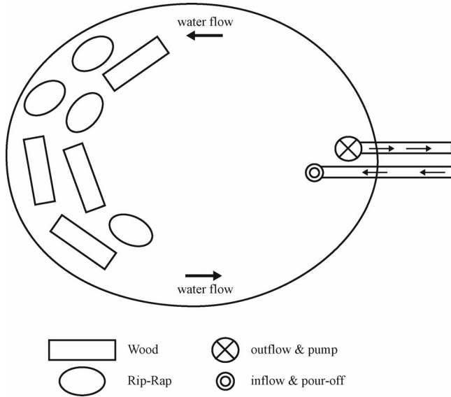
FIG. 2.—Diagram of one 1135 L mesocosm showing inflow and outflow of water and placement of spawning substrates (substrate was placed randomly, see text); a 1500 L/h powerhead pump was hung off the outflow and directed flow in the mesocosm
