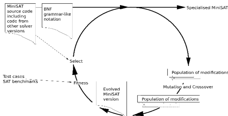
Fig. 1. Overview of the Genetic Improvement framework used.
