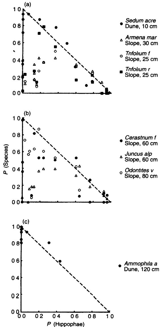
Fig 5 Probability of occurrence of several early successional species plotted against the probability of occurrence of Hippophae rhamnoides of an estimated minimal plant height h . The broken lines indicate the relationship P(\text{species}) = 1 - P(\text{Hippophae above height } h) . Each species is plotted when its maximal height (see legend) was comparable with the minimal height h of Hippophae . Height h of Hippophae : (A) 31 cm (1 year old), (B) 57 cm (2 years old) and (C) 108 cm (5 years old).
