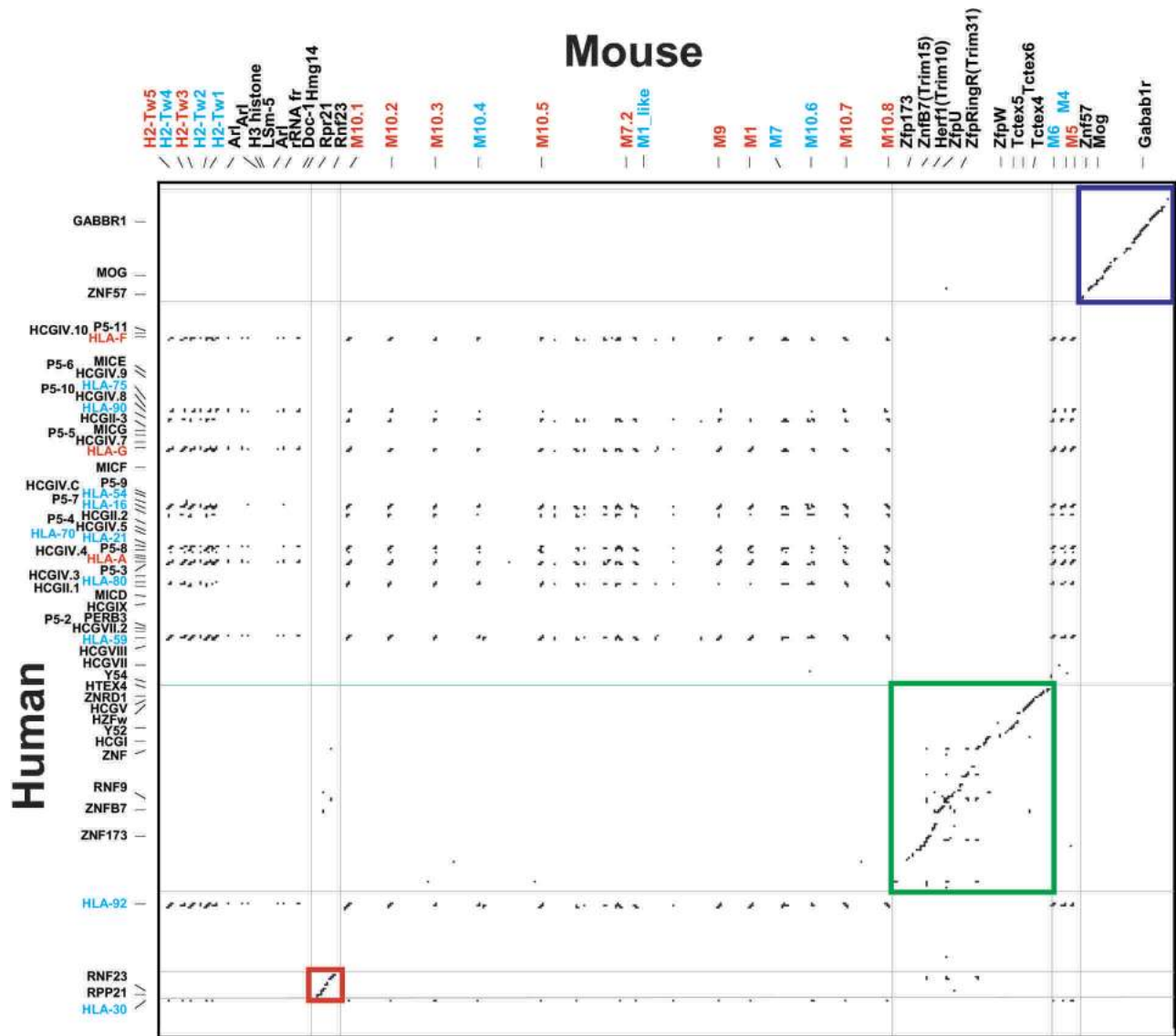
Figure 5 Dot matrix analysis of the telomeric class I region of mouse and man. The 951,695-bp sequence of the centromeric H2-M region is compared with 853,185 bp of the HLA region (accession no. NF_001520). Class I genes are red, class I pseudogenes are blue; other genes and pseudogenes are black. The red, green, and blue boxes mark the three framework regions that are conserved syntenic regions of orthologous nonclass I genes, which yield clear diagonal lines on the dot matrix. The class I genes give only short lines of similarity between paralogous genes.
