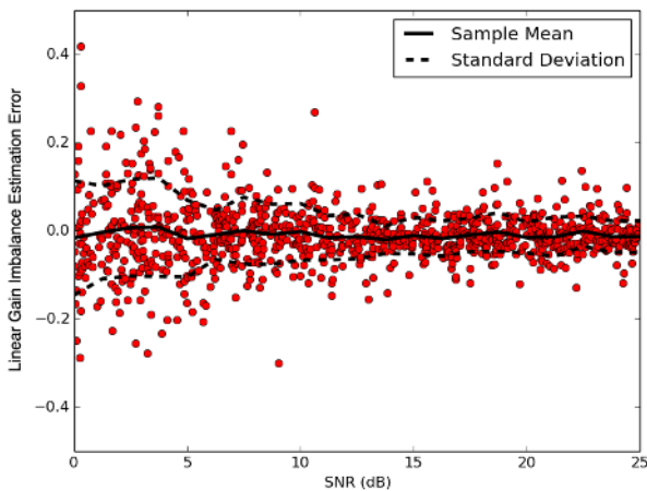
FIGURE 13. The linear gain imbalance estimation errors for signals simulated with SNRs between 0dB and 25dB. True linear gain imbalances vary uniformly between [-0.9, 0.9] .
