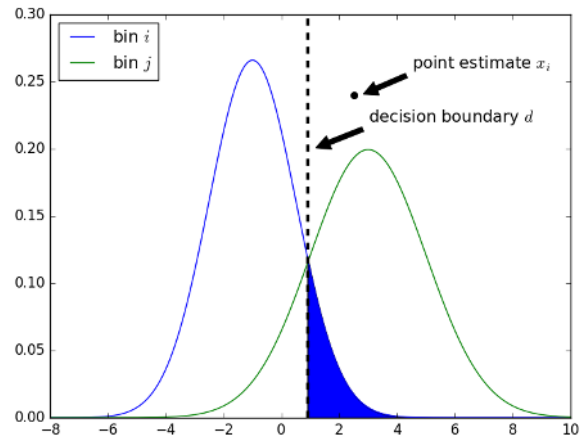
FIGURE 23. An example decision scenario.
