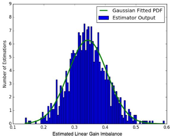
FIGURE 22. The fitted Gaussian curve for the 1024 input CNN gain imbalance estimator output histogram with PSK input signals at 10dB SNR (Linear gain imbalance = 0.30).
