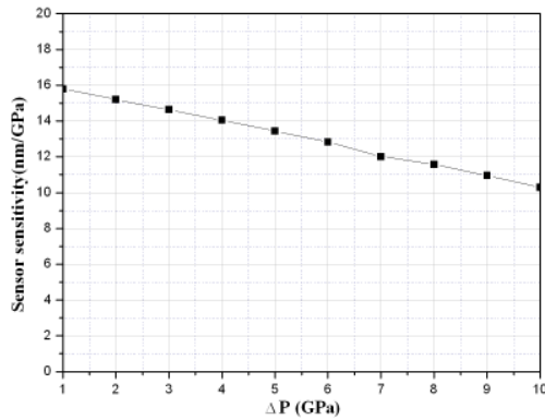
Fig. 5. Sensitivity s variation with a change of pressure.
