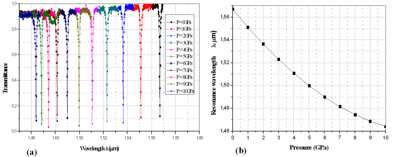
Fig. 4. (a) Transmittance for different applied pressure within the range 0–10 GPa. (b) The pressure vs. the output drop wavelength.
