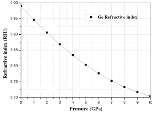
Fig. 2. Ge refractive index as a function of pressure.
