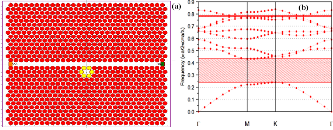
Fig. 1. (a) The designed pressure sensor, (b) calculated photonic band gap.
