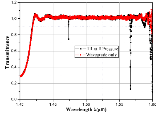
Fig. 3. Transmittance of the sensor at 0 pressure.
