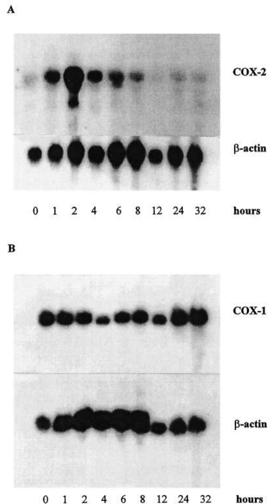
FIGURE 1. COX-2 is the inducible COX isoform in 3LL tumor cells. Following IL-1 \beta stimulation of 3LL cells, Northern blot analysis was performed with COX-2 (A) and COX-1 (B) cDNA probes. Maximal COX-2 mRNA expression occurred 2 h after incubation with IL-1 \beta , whereas COX-1 mRNA expression remained unchanged.
