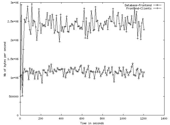
Figure 20. Bulletin board network usage in bytes/s as a function of time at the peak throughput for the browsing mix.
