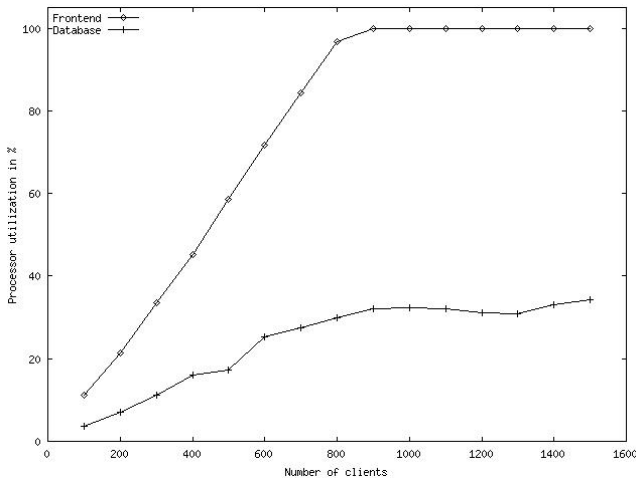
Figure 10. Auction site percentage CPU utilization as a function of number of clients for the browsing mix.
