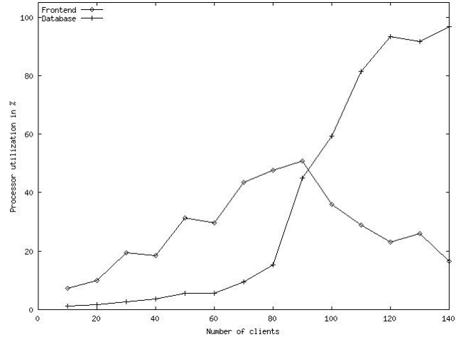
Figure 5. Online bookstore percentage CPU utilization as a function of number of clients for the ordering mix.
