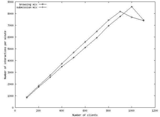
Figure 15. Bulletin board throughput in interactions per minute as a function of number of clients.
