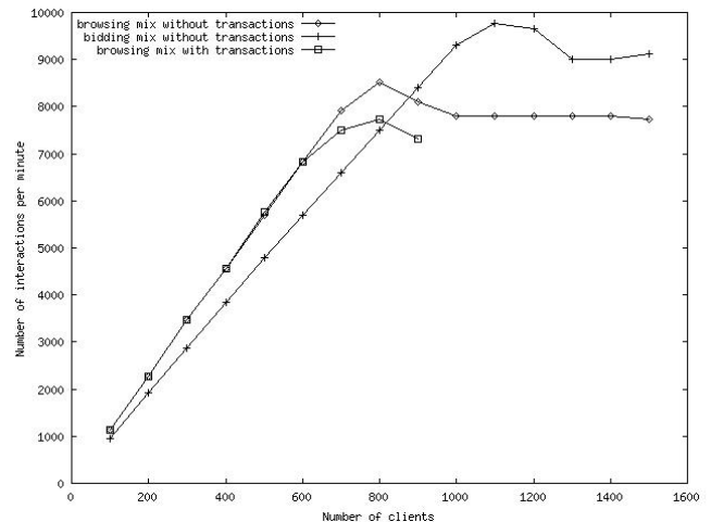
Figure 9. Auction site throughput in interactions per minute as a function of number of clients.
