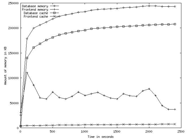
Figure 12. Auction site memory usage in KB as a function of time at the peak throughput for the browsing mix.
