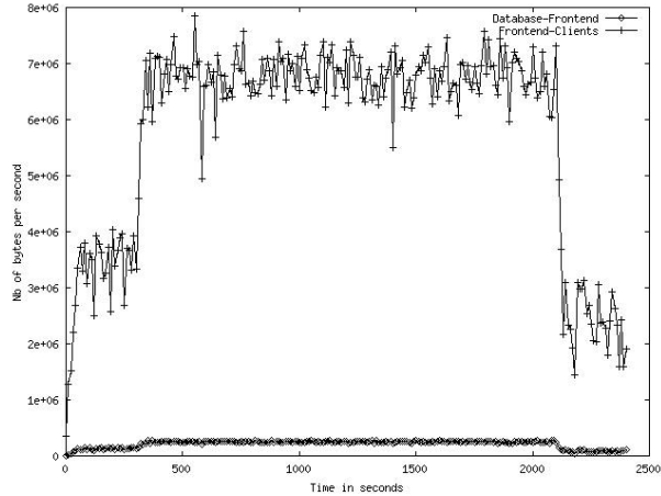
Figure 14. Auction site network usage in bytes/s as a function of time at the peak throughput for the browsing mix.
