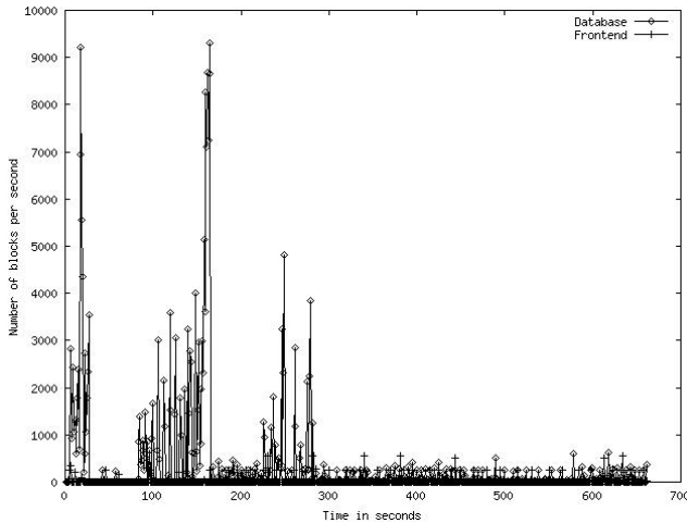
Figure 7. Online bookstore disk usage in number of blocks per seconds as a function of time at the peak throughput for the ordering mix.
