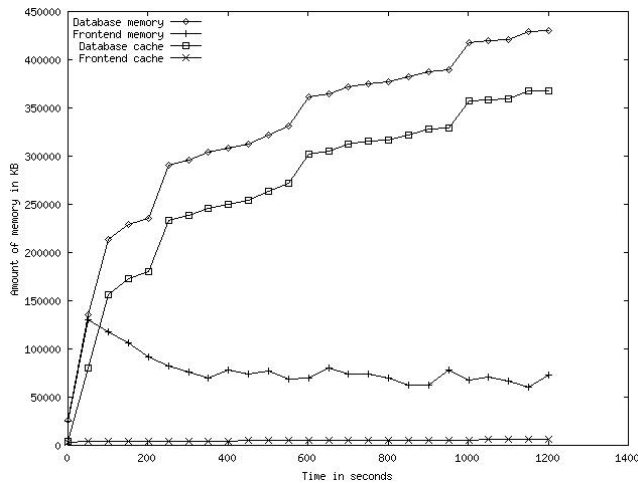
Figure 18. Bulletin board memory usage in KB as a function of time at the peak throughput for the browsing mix.
