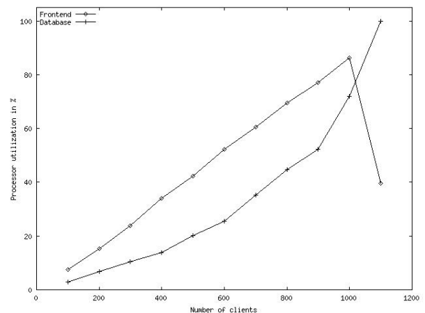
Figure 17. Bulletin board percentage CPU utilization as a function of number of clients at the peak throughput for the submission mix.
