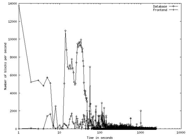
Figure 13. Auction site disk usage in number of blocks per second as a function of time (x-axis is log-scale) at the peak throughput for the browsing mix.
