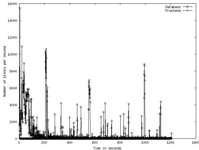
Figure 19. Bulletin board disk usage in number of blocks per second as a function of time at the peak throughput for the browsing mix.
