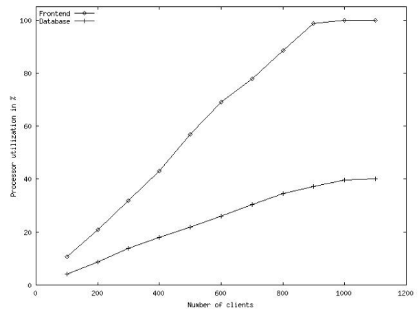
Figure 16. Bulletin board percentage CPU utilization as a function of number of clients at the peak throughput for the browsing mix.
