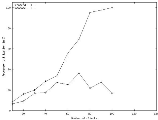
Figure 4. Online bookstore percentage CPU utilization as a function of number of clients for the shopping mix.
