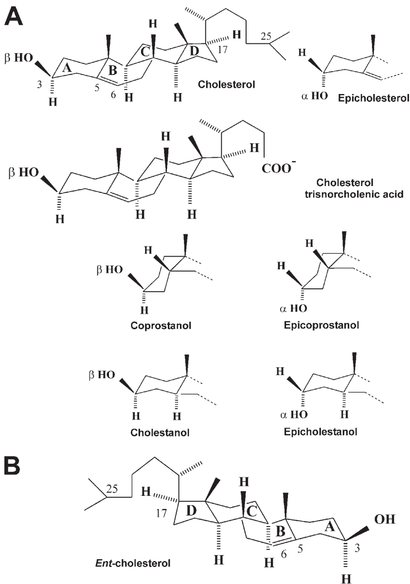
Figure 1. Molecular structures of cholesterol and analogues. (A) Structures of cholesterol and cholesterol trisnorcholelic acid are shown in full. Only the steroid nucleus around the A/B fusion is shown for the remaining compounds to emphasize differences in the planar orientation of the C3 hydroxyls and geometry of the A/B ring fusion. The free carboxyl group ( pK_a = 5.5 ) at the end of the side chain in cholesterol trisnorcholelic acid is shown in its ionized form, which likely predominates under our experimental conditions ( pH = 7.2 ). (B) The structure of cholesterol enantiomer ( ent -cholesterol) is shown in full to emphasize that this molecule is a mirror image of cholesterol. For all compounds, trivial names are provided. For IUPAC nomenclature, please refer to Table I.
