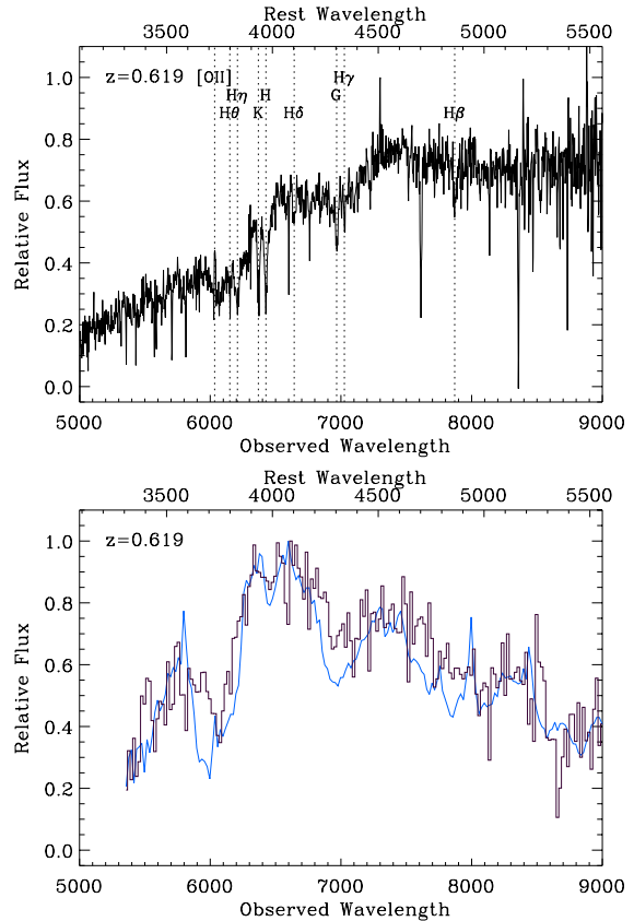
Fig. 6.— (Upper) Unsmoothed spectrum of SN 1997J showing the narrow lines used to determine the redshift. (Lower) rebinned spectrum of SN 1997J (histogram) after subtraction of template S0 host galaxy, compared with SN 1999bn at day +2 (smooth curve).
