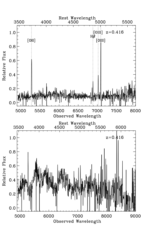
Fig. 15.— (Upper) Unsmoothed spectrum of the host of SN 1997am showing the narrow lines used to determine the redshift. (Lower) lightly smoothed spectrum of SN 1997am.
