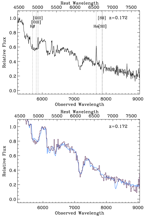
Fig. 5.— (Upper) Unsmoothed spectrum of SN 1997I obtained at the ESO 3.6m showing galaxy lines used to determine the redshift. (Lower) Re-binned spectrum of SN 1997I (histogram) after interpolating over narrow galaxy lines and subtraction of an Sb template galaxy spectrum, compared with SN 1999bp at +1 day (smooth curve).
