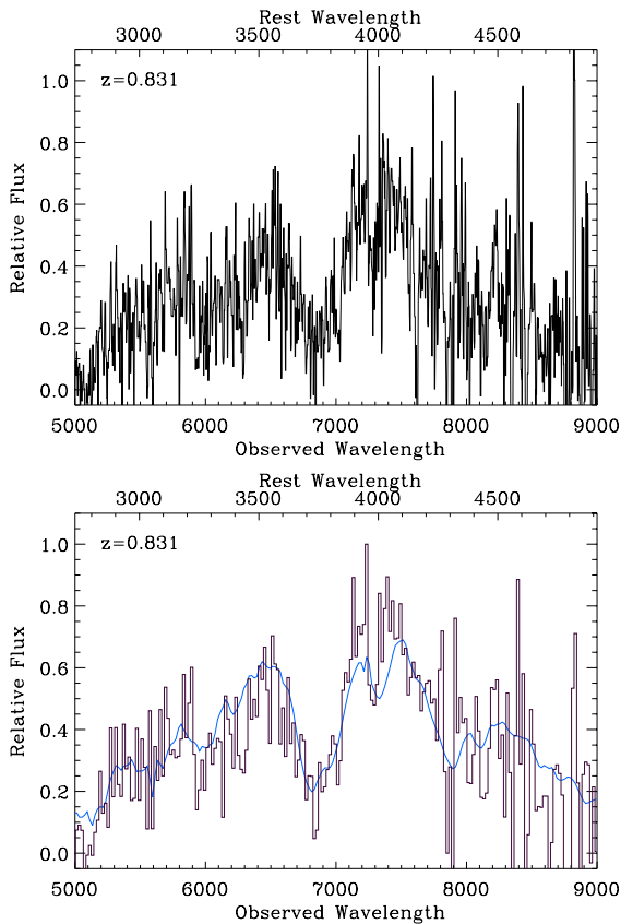
Fig. 16.— (Upper) Lightly smoothed spectrum of SN 1997ap. (Lower) Rebinning spectrum of SN 1997ap (histogram) after interpolating across the sky absorption region at 7600\text{\AA} compared with the Type Ia SN 1989B at -5 days (smooth curve).
