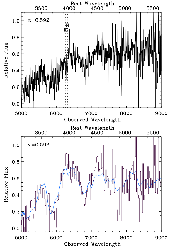
Fig. 12.— (Upper) Lightly smoothed spectrum of SN 1997ag showing narrow features used to determine the redshift. (Lower) rebinned spectrum of SN 1997ag (histogram) after interpolating across narrow galaxy lines, compared with the Type Ia SN 1990N at +7 days before maximum (smooth curve).
