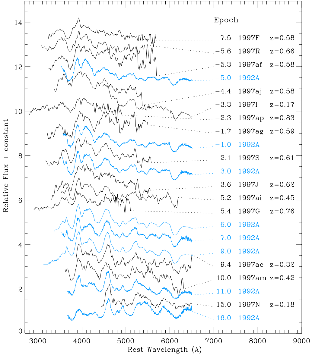
Fig. 17.— The time sequence of high redshift supernova spectra in order of rest-frame date relative to maximum light, as determined from the light curve ( \pi_c ). Spectra of the nearby Type Ia, SN 1992A are interspersed for comparison.
