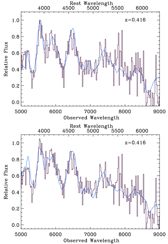
Fig. 15.— cont. (Upper) Rebinned spectrum of SN 1997am (histogram) after interpolating across cosmic rays and narrow lines from the host galaxy and subtraction of a SB1 galaxy template, compared with the Type Ia SN 1992A at +9 days (smooth curve). (Lower) previous plot but with the Type Ia SN 1991T at +10 days for comparison.
