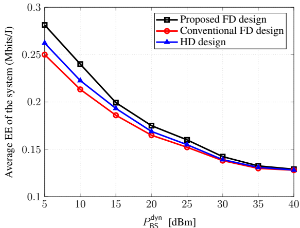
Fig. 9. EE versus P_{\text{BS}}^{\text{dyn}} where we set P_{\text{BS}}^{\text{dyn}} = \xi P_{\text{BS}}^{\text{dyn}}, \forall \ell and \xi = 0.7 , with N = M = 4, K = L = 3, \rho = -40 dB, \bar{r}_u = 1 Mbits/s.
