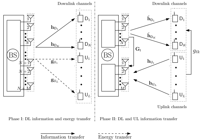
Fig. 1. A WPCN system with WET in the downlink channel and WIT in both uplink and downlink channels.
