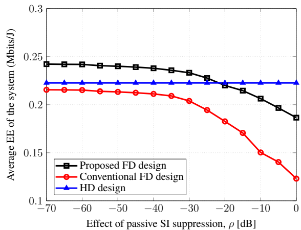
Fig. 8. EE versus \rho with N = M = 4 , K = L = 3 , \bar{r}_u = 1 Mbits/s.
