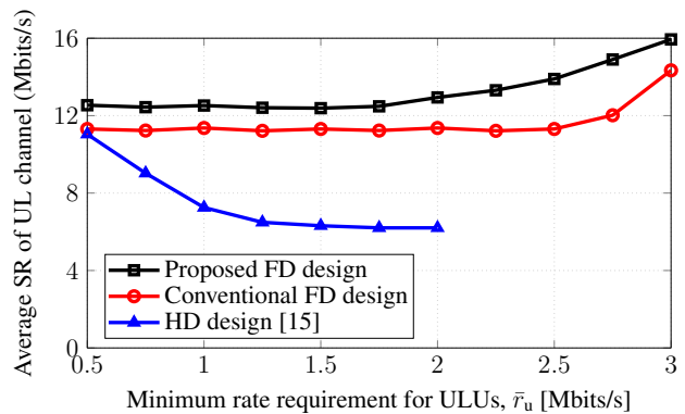
(a) SR of UL channel.
