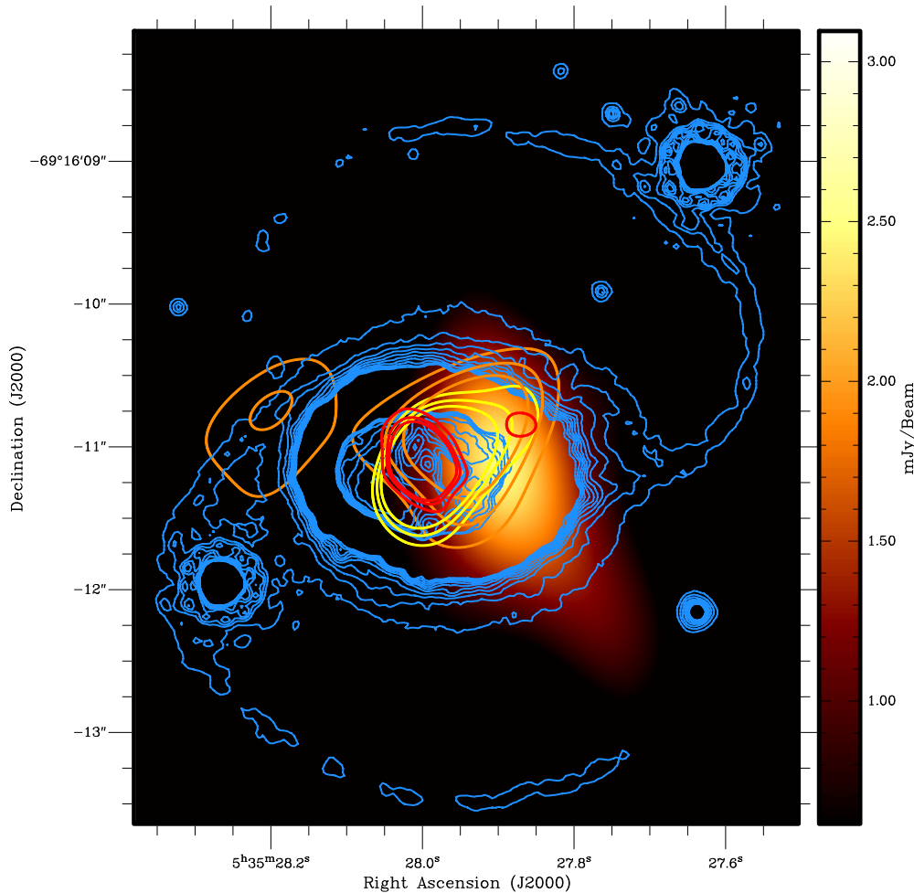
Figure 5. Comparison of the diffraction-limited images of SNR 1987A at 102, 213, and 345 GHz, as obtained after subtraction of the scaled model flux density at 44 GHz (see Figure 1, right column), with the optical image of the remnant. In detail, the residual image at 102 GHz (brown–yellow color scale) is overlaid with the contours outlining the residual images at 213 GHz (orange) and at 345 GHz (yellow). To locate the main sites associated with dust emission, the diffraction-limited image at 672 GHz is also outlined (red; as from Figure 1, left column). Images at 213, 345, and 672 GHz are overlaid with contours at 3\sigma , 4\sigma , and 5\sigma flux density levels. The angular beams associated with each image, as shown in Figure 1, are listed in Table 2. The HST image (Larsson et al. 2011) is outlined via contours (blue) that highlight the structure of the outer rings, the equatorial ring, and the ejecta.
