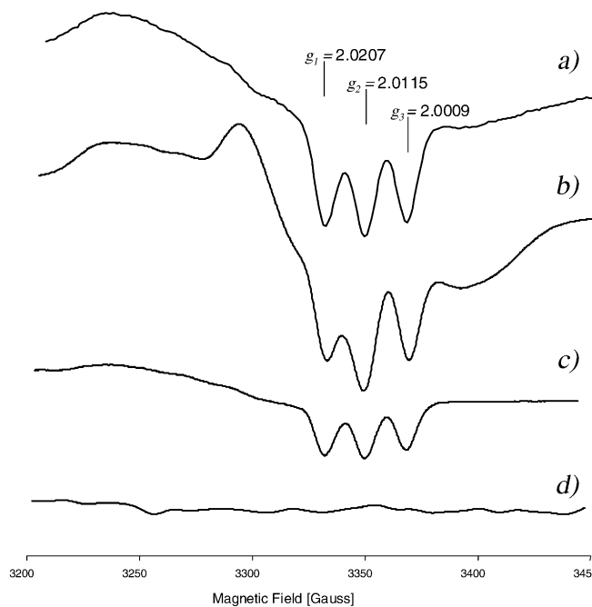
Fig. 1 Electron spin resonance spectra of dry-cured meat products (Parma and Serrano ham), cooked brine-cured ham and pure nitrosylmyoglobin recorded at 150 K. Spectrum a Nitrosylmyoglobin (0.20 mM), b Serrano ham (nitrate added during curing), c Cooked, brine-cured ham (60 ppm nitrite added during curing) and d Parma ham (only NaCl added)
