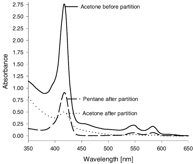
Fig. 5 UV/visible spectra of acetone/water (75%/25%) extracts of pigments from mature, dry-cured Parma (18 months) followed by separation into 2:1 (v/v) pentane added aqueous 4% NaCl
