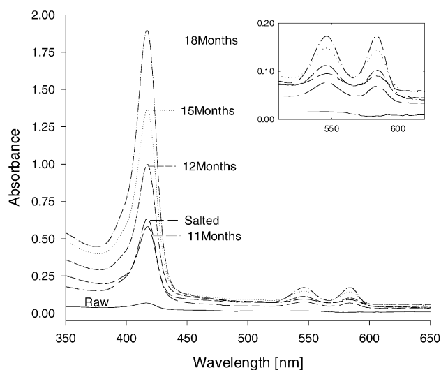
Fig. 4 UV/visible spectra of acetone/water (75%/25%) extracts of pigments from raw pork leg, salted ham and dry-cured Parma ham at 4 different processing stages obtained within 2 h of extraction and recorded at 25 °C temperature. Inset shows \beta - and \alpha -bands in detail
