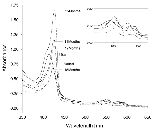
Fig. 3 UV/visible spectra of pigments extracted from raw pork leg, salted ham and dry-cured Parma ham at 4 different processing stages by 0.20 M aqueous phosphate buffer obtained within 2 h of extraction and recorded at 25 °C. Inset shows \beta - and \alpha -bands in detail
