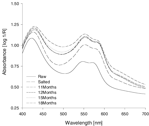
Fig. 2 Visible region of visible/near-infrared reflectance spectra of raw pork leg, salted ham and dry-cured Parma ham at 4 different processing stages recorded at 25 °C using a "spinning cup" cell (sampling area=12.5 cm 2 )
