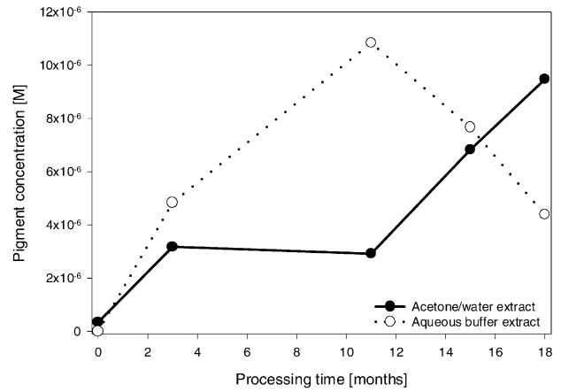
Fig. 6 Changes in concentration of red pigments present in aqueous buffer and acetone/water extract of dry-cured Parma ham during the course of processing. Samples for 12 months maturation are omitted from the plot for purpose of clarity. Estimation of concentration is based on Soret band absorbance and extinction coefficients (see Table 1) for the two respective Parma ham extracts
