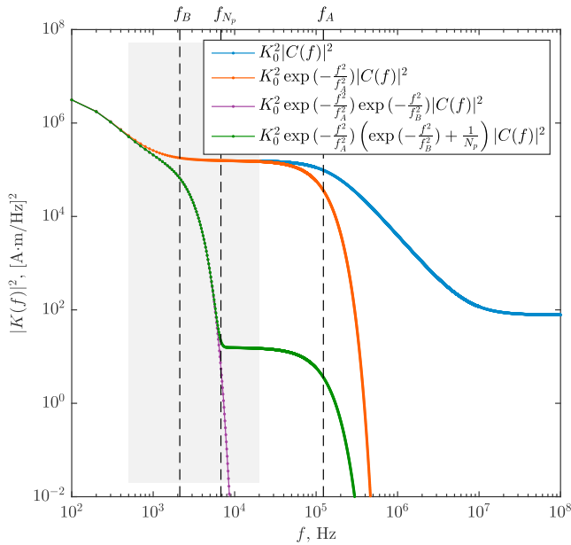
Figure 2. Energy spectrum of the TGF source current moment. Blue line: the spectrum of the total current composition in case if all N_{TGF} runaway electrons ran instantaneously. Red line: if all runaway electrons ran in a single avalanche (modulation of the spectrum by a single RREA and a seeding pulse spectrum). Purple line: modulation by the spectrum of the TGF time profile at source. Green line: all runaway electrons are organized into N_p = 10^4 avalanches. Three characteristic frequencies f_A , f_B , and f_{N_p} are shown as black vertical dashed lines. The frequency range of the observed VLF sferics is highlighted by the gray background rectangle (500 Hz to 20 kHz).
