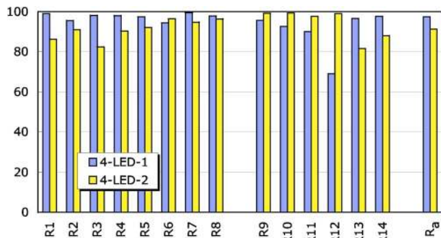
Fig. 8 Special CRI of the four-chip white LED models shown in Fig. 7.
