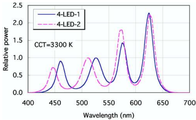
Fig. 7 The SPDs of the two four-chip white LED models 4-LED-1 and 4-LED-2.
