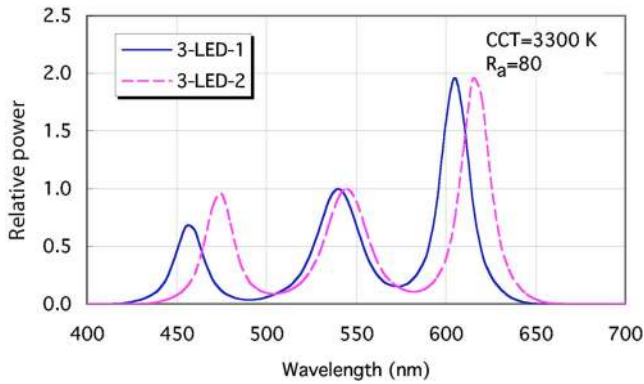
Fig. 4 The SPDs of the two three-chip LED models, both having R_a=80 at 3300 K.
