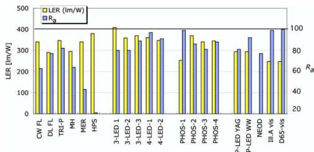
Fig. 3 LER and the general CRI R_a of the conventional sources and LED models analyzed.
