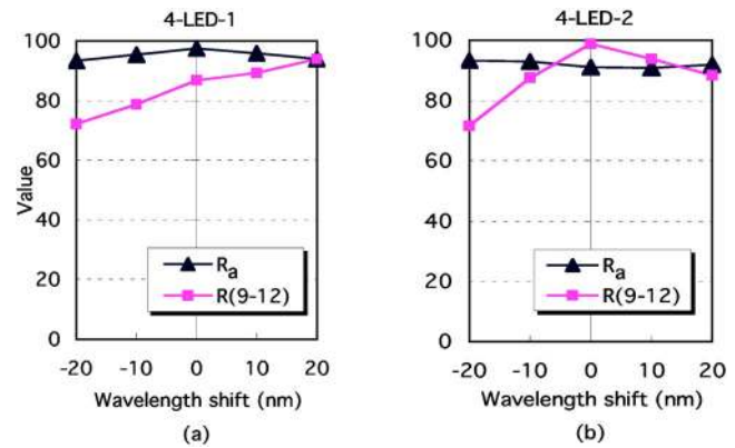
Fig. 9 The changes of R_a and R(9-12) of the four-chip LED models when the wavelengths of the sample spectral reflectance data are shifted.
