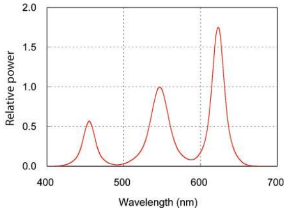
Fig. 13 The SPD of a three-chip white LED model with peak wavelengths 455, 547, and 623 nm.
