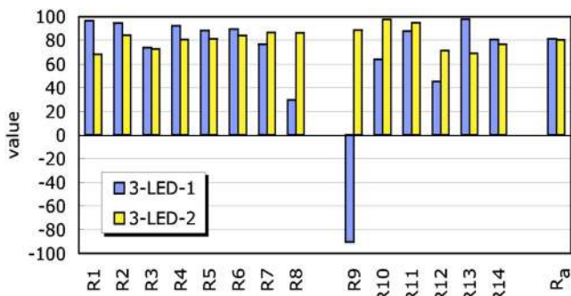
Fig. 5 Special CRI of the two three-chip white LED models shown in Fig. 4.
