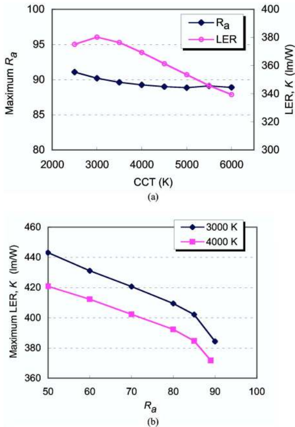
Fig. 2 Examples of optimization of RGB white LED spectra. The peak wavelengths of LEDs range from 452 to 472 nm for blue, from 543 to 553 nm for green, and from 598 to 620 nm for red. \Delta\lambda_{0.5}=20 nm except for green (30 nm). (a) Maximum R_a obtained at varied CCT. (b) Maximum LER, K (lm/W), obtained at varied R_a .
