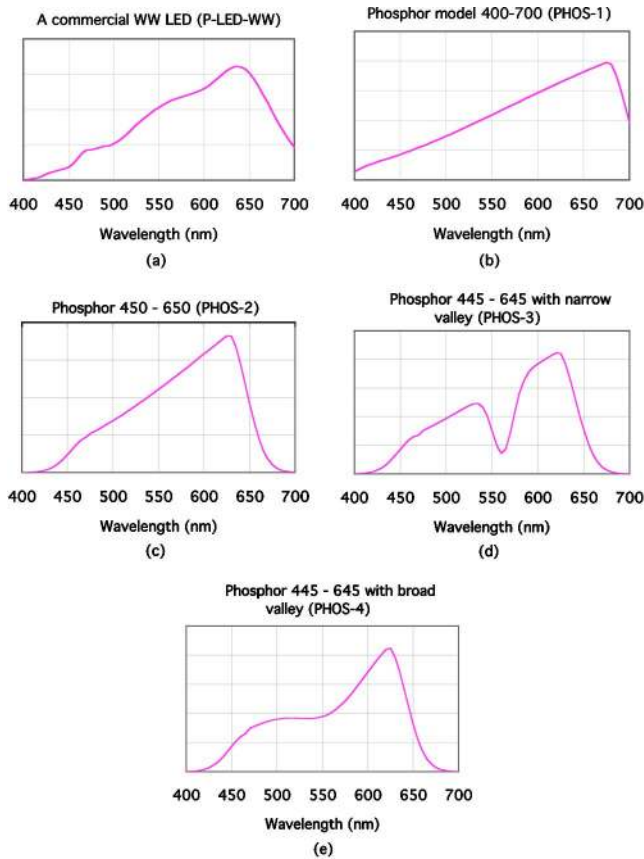
Fig. 10 SPDs of (a) commercially available warm white LED model and (b to e) phosphor-type LED models.
