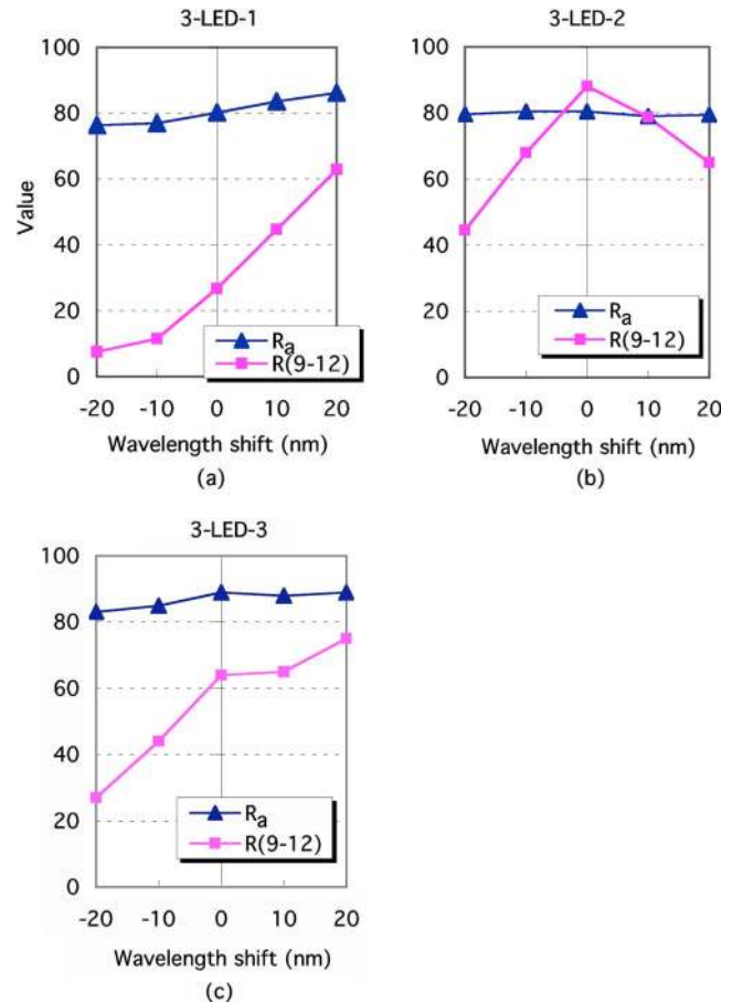
Fig. 6 The changes of R_a and R(9-12) for three-chip white LED models when the wavelengths of the sample spectral reflectance data are shifted.
