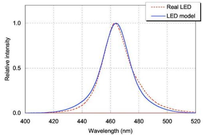
Fig. 1 LED model S_{LED}(\lambda) at 464 nm compared with the SPD of a typical real blue LED.
