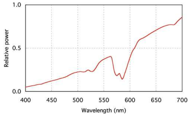
Fig. 11 The SPD of an incandescent lamp with neodymium glass.
