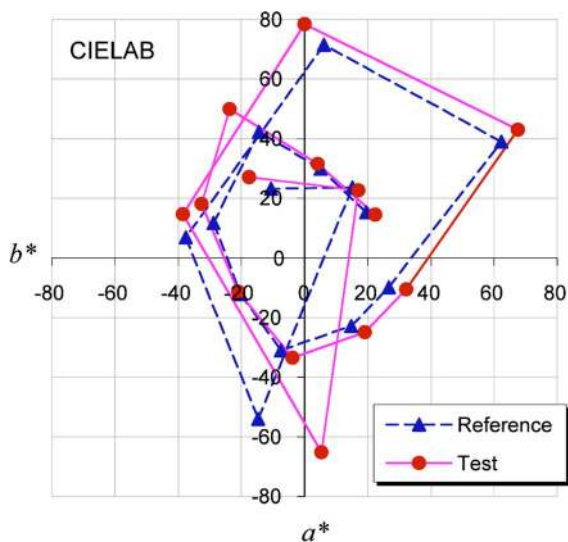
Fig. 14 Colors of the 14 samples in CIELAB space under illumination by the three-chip LED model shown in Fig. 13 and by the reference source (Planckian).
