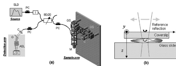
Fig. 1. (a) Schematics of the SD-OCPM system: SLD, superluminescent diode; PCs, polarization controllers; I, isolator; 80/20, 80/20 fiber-based beam splitter; G, transmission grating; ASL, three-element air-spaced lens; LSC, line scan camera; C, collimator; GS, galvanometer scanner; M, microscope objective. (b) Sample placed between a coverslip and a microscope slide. SD-OCPM measures phase distribution of a sample referenced to the top surface of the coverslip.
