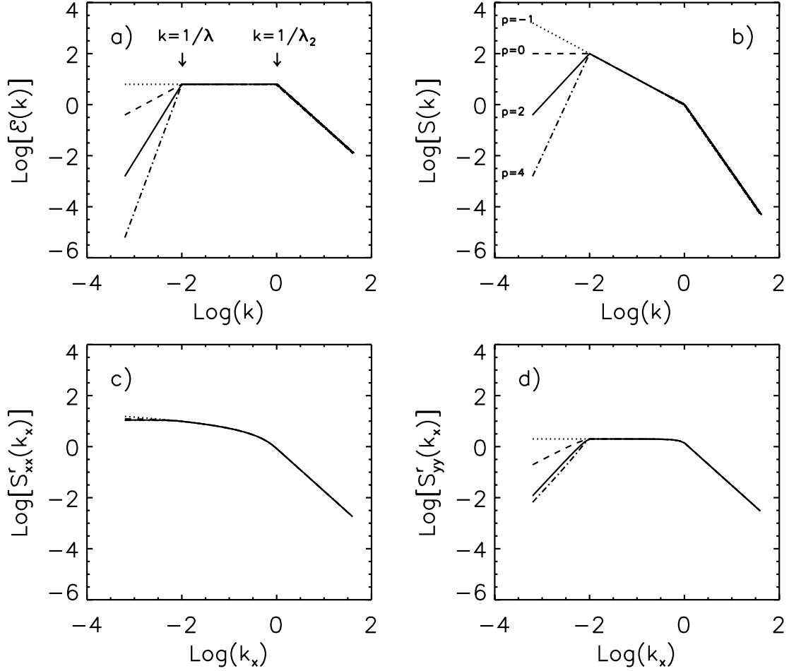
FIG. 1.— Example of axisymmetric 2D magnetic power spectra with two length scales: \lambda_2 , the 2D bendover scale, and \lambda , which marks the onset of long-wavelength (low-wavenumber) behavior. Here S(k) is specified by eq. (26) for p = -1 (dotted lines), p = 0 (dashed lines), p = 2 (solid lines), and p = 4 (dash-dotted lines), with C\langle b^2 \rangle = 1 , \nu = -5/3 , \lambda_2 = 1 , and \lambda = 100 . (a) Omnidirectional energy spectrum, \mathcal{E}(k) ; (b) modal spectrum, S(k) ; (c) longitudinal reduced spectrum, S'_{xx}(k_x) ; and (d) transverse reduced spectrum, S'_{yy}(k_x) .
