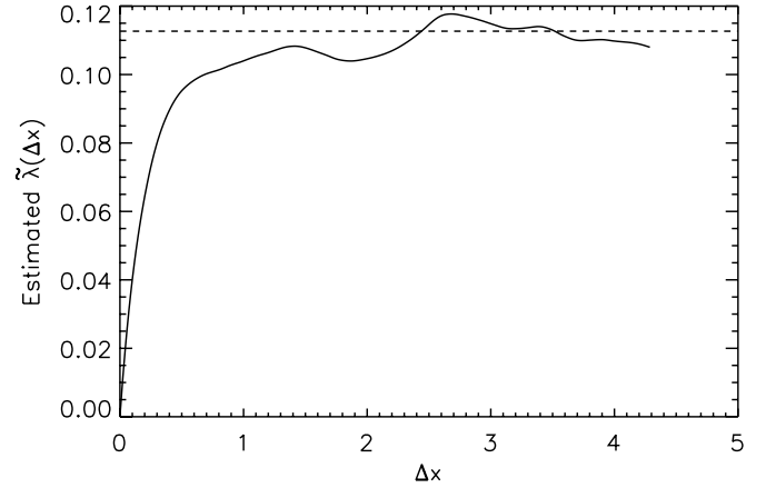
FIG. 2.—Results of evaluation of the ultrascale \tilde{\lambda} from data extracted from a 1024 \times 1024 2D spectral MHD simulation (solid line). This confirms that at large \Delta x , the estimate does tend to the exact value of the ultrascale for the known power spectrum, \tilde{\lambda} = 0.11267 (dashed line). To calculate the flux integrals, samples of b_y(x, y_0) were taken for 1024 values of x at each of 20 values of y_0 . Note that the simulation box size is 2\pi and the correlation scale is 0.05 for this data set.
