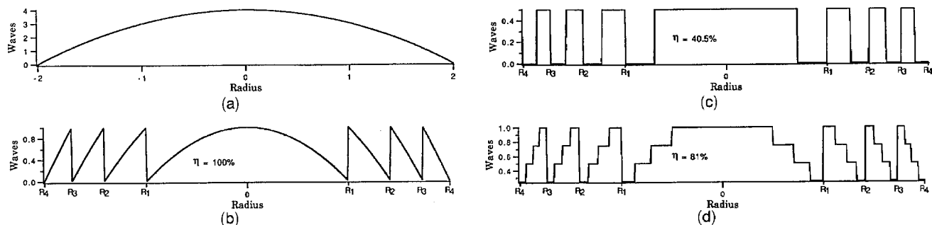
Fig. 1. Diffraction lens construction: (a) conventional refractive lens, (b) diffractive lens with continuous quadratic blaze profile, (c) phase-reversal (or Wood) lens, (d) four-level approximation to quadratic blaze profile.
