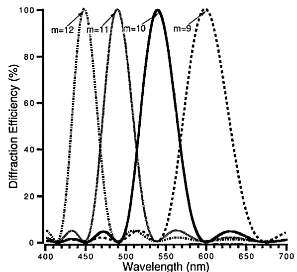
Fig. 2. Diffraction efficiency of the m th diffracted order versus wavelength for a MOD lens with p = 10 .
