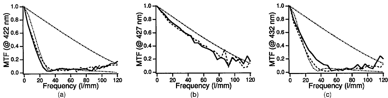
Fig. 5. MTF for p = 2 and m = 3 . The design wavelength, 427 nm, is represented in (b) and a wavelength detuning of \pm 5 nm is represented in (a) and (c). The diffraction limit is the same in all three cases. The tangential MTF is displayed by a dashed curve, and the sagittal MTF is illustrated by a solid curve. The theoretical tangential performance at 422 and 432 nm is also illustrated as a dotted-dashed curve.
