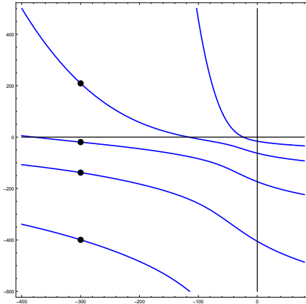
Figure 8. The dots represent the points (x_0, x_3^{(n)}) = (-300, -e^{E_n}) , n = 1, 2, 3, 4 , giving the spectrum of the operator \mathcal{O}_2 with a negative value of x_0 = -300 .
