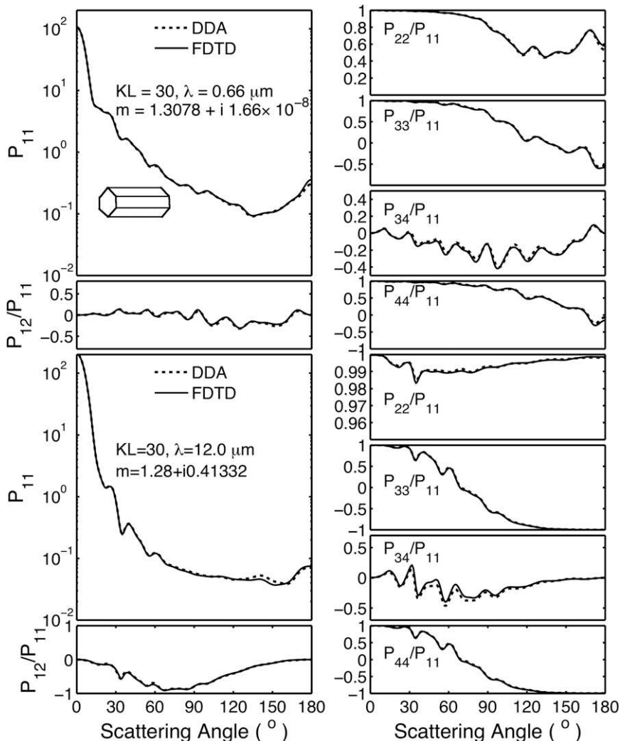
FIG. 4. Comparison of the phase matrix elements from the FDTD and the ADDA at the wavelengths of 0.66 and 12 \mu\text{m} .
