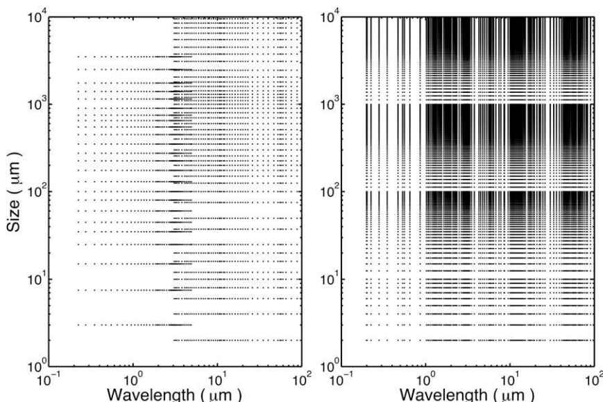
FIG. 2. Grid points in the computational domain of the particle size and the wavelength. (left) The previous databases. (right) The present database.
