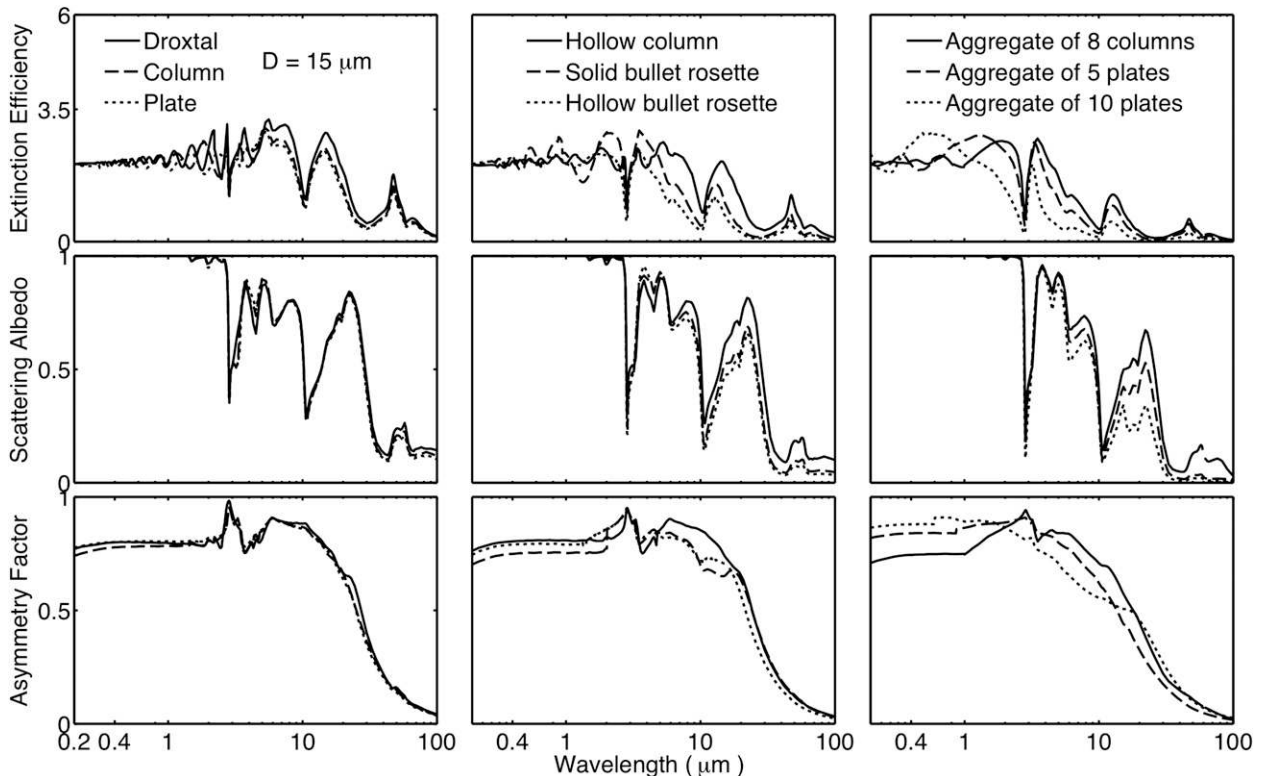
FIG. 8. Spectral variation of the extinction efficiency, the single-scattering albedo, and the asymmetry factor at the particle maximum dimension of 15 \mu\text{m} .
