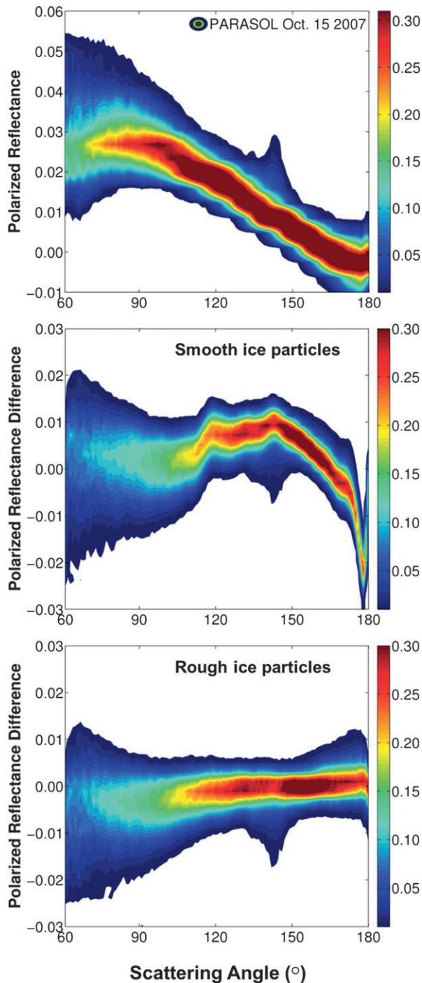
FIG. 15. (top) Density contours of polarized reflectance measurements at 865 nm from the PARASOL satellite on 15 Oct 2007. Over 60 000 pixels over the ocean are included, corresponding to approximately 866 000 total viewing geometries plotted. (middle) The difference between simulated polarized reflectance and measured polarized reflectance for each viewing geometry. The MODIS Collection 5 habit distribution and smooth ice particles with an effective diameter of 50\ \mu\text{m} were used in the simulation, and the optical depth was 5. (bottom) The difference in polarized reflectance using C5 with severely roughened ice particles and all simulation parameters the same as (middle).
