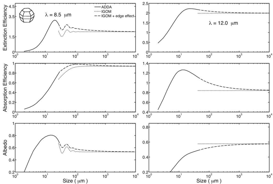
FIG. 7. Edge/tunneling effect contribution to the extinction efficiency, the absorption efficiency, and the single-scattering albedo.
