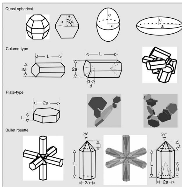
FIG. 3. Ice crystal habits: quasi-spherical, column-type, plate-type, and bullet rosette particles.
