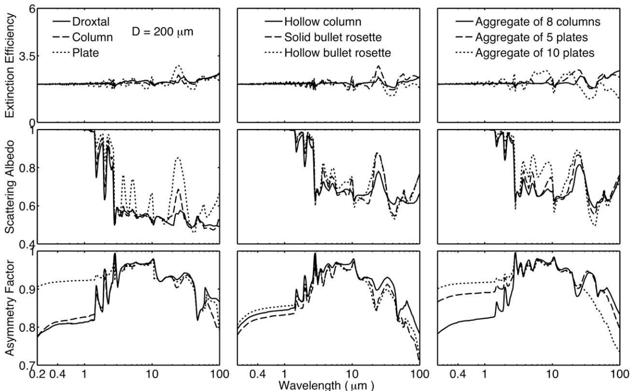
FIG. 9. As in Fig. 8, but for the particle maximum dimension of 200 \mu\text{m} .
