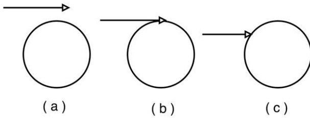
FIG. 6. Ray types: (a) edge rays, (b) grazing rays, and (c) rays incident on the particle.
