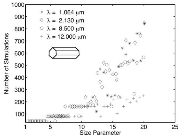
FIG. 5. Number of ADDA simulations (or particle orientations specified by \beta and \gamma ) at four representative wavelengths in the hexagonal columns case.
