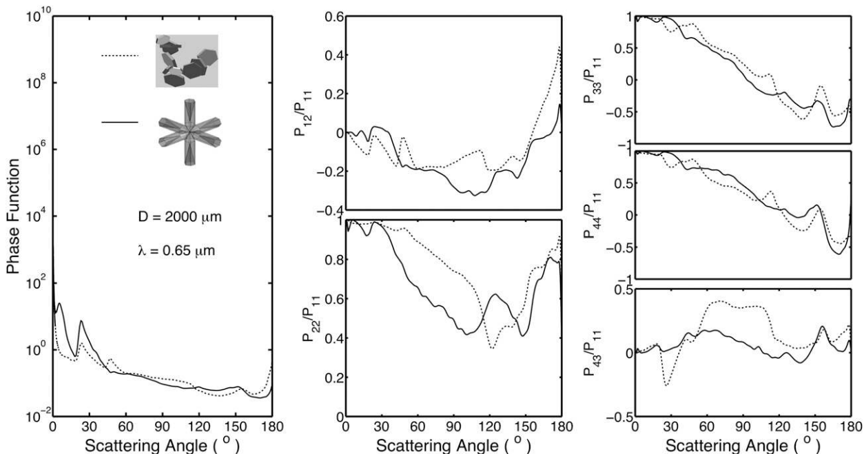
FIG. 12. As in Fig. 11, but for the size of 2000 \mu\text{m} .
