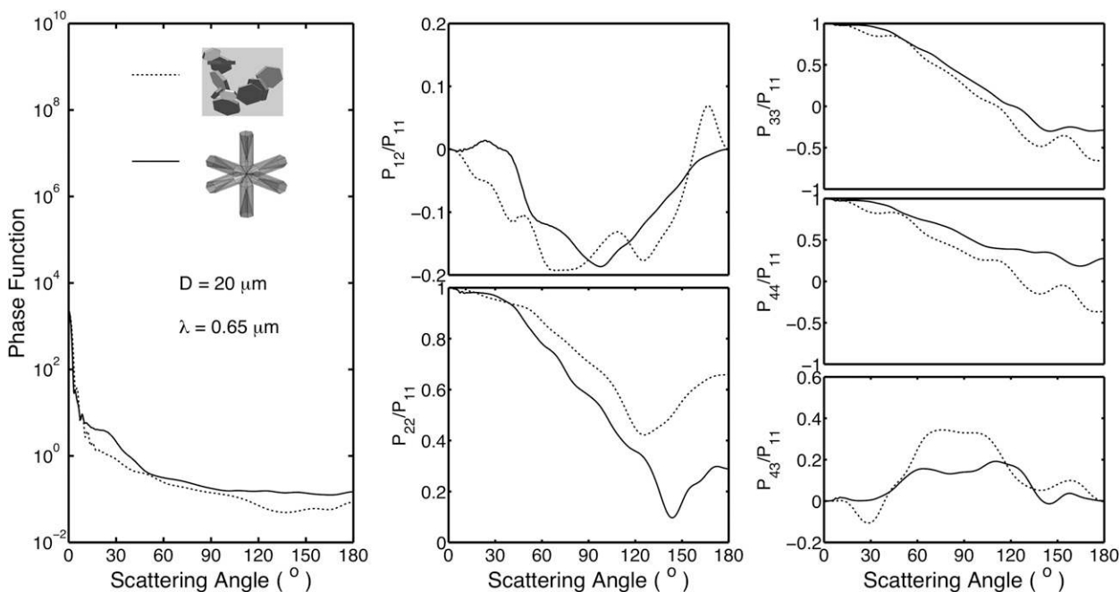
FIG. 11. Comparison of the phase matrix elements for an aggregate of 10 plates and a hollow bullet rosette at the size of 20 \mu\text{m} .
