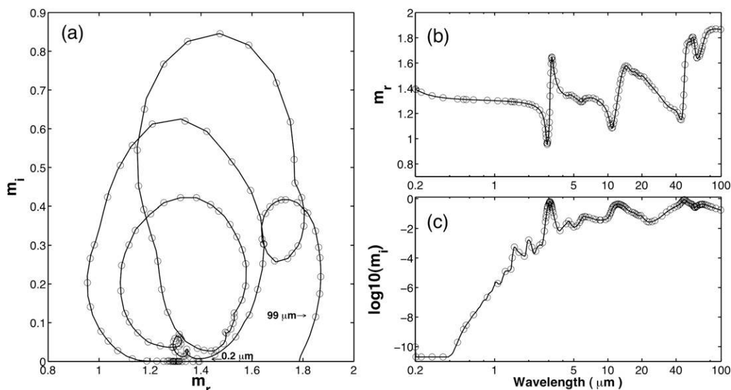
FIG. 1. (a) Correlation of the real and imaginary part of the refractive index. (b) Real part of the refractive index. (c) Imaginary part of the refractive index.
