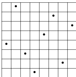
Figure 1. An 8-Rook Sampling Design in Two Dimensions
