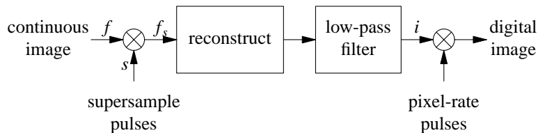
Figure 2. Conversion of Ray-Casting Samples into Pixels
