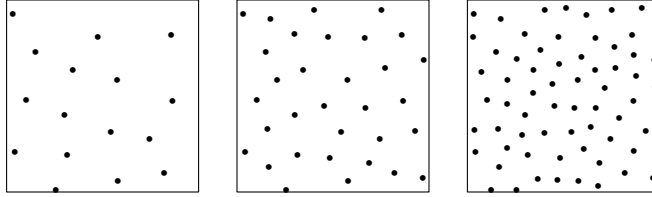
Figure 4. Sequential Generation of High-Frequency Samples
