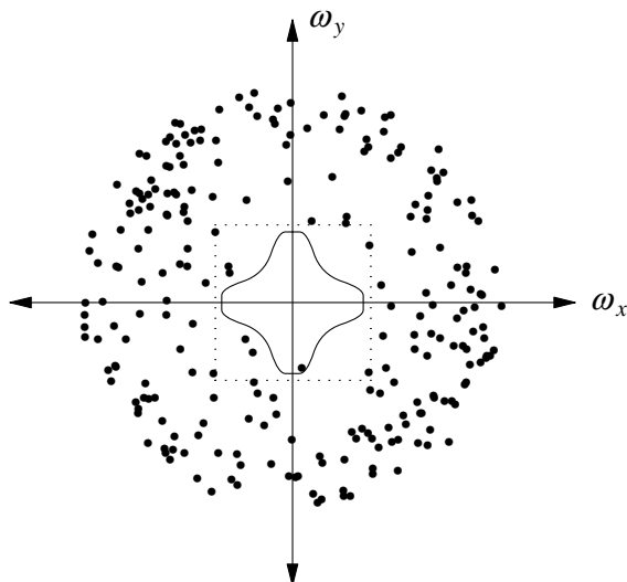
Figure 3. Spectrum of Nonuniformly Sampled Image
