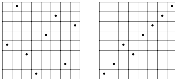
Figure 15. 8-Rook Sampling Patterns
