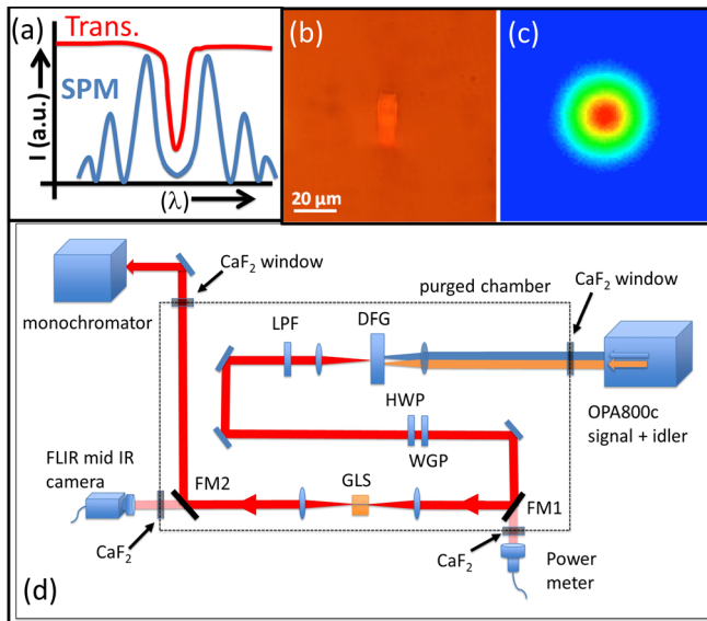
FIG. 1. The concept of using self-phase modulation to reshape a pulse spectrum (SPM) around an absorption feature (Trans.) is shown in (a). The GLS waveguide facet is shown in (b) and corresponding mode image (c) at 4260 nm on the same scale. (d) Experimental arrangement for the coupling of mid infrared pulse train into GLS waveguide. The signal and idler outputs from an OPA source are focused inside a difference frequency generation (DFG) crystal. LPF, long pass filter; HWP, half wave plate; WGP, wire grid polarizer; FM1 and FM2 are flip mirrors.
