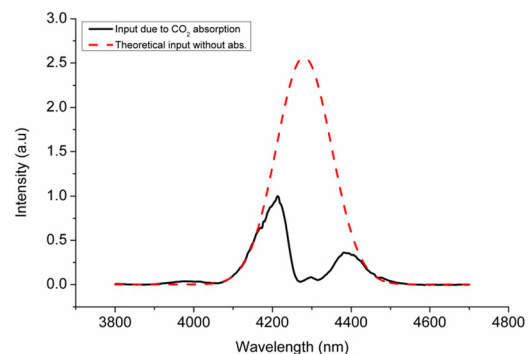
FIG. 2. Input pulse spectrum centered on 4260 nm that has been shaped by atmospheric \text{CO}_2 absorption (solid line). The fitted unmodified spectrum (broken line).
