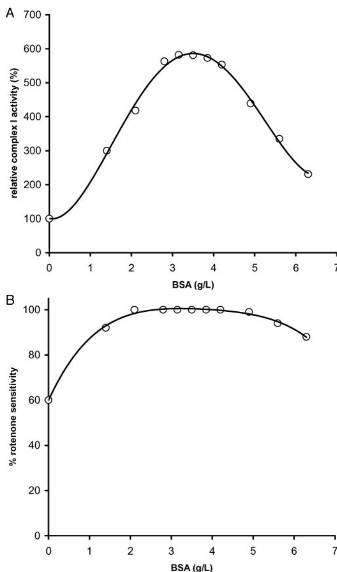
Fig. 1. (A), effect of BSA on relative rotenone-sensitive complex I activity in muscle mitochondrial suspensions.
