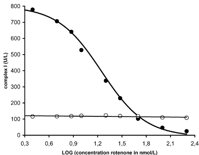
Fig. 2. Inhibition of complex I activity by rotenone measured in muscle mitochondria.
