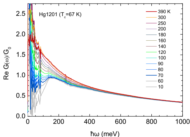
Fig. 1. Optical sheet conductance of underdoped Hg1201 ( T_c = 67 K). Temperatures from 10 to 390 K. Data below T_c are shown in gray.
