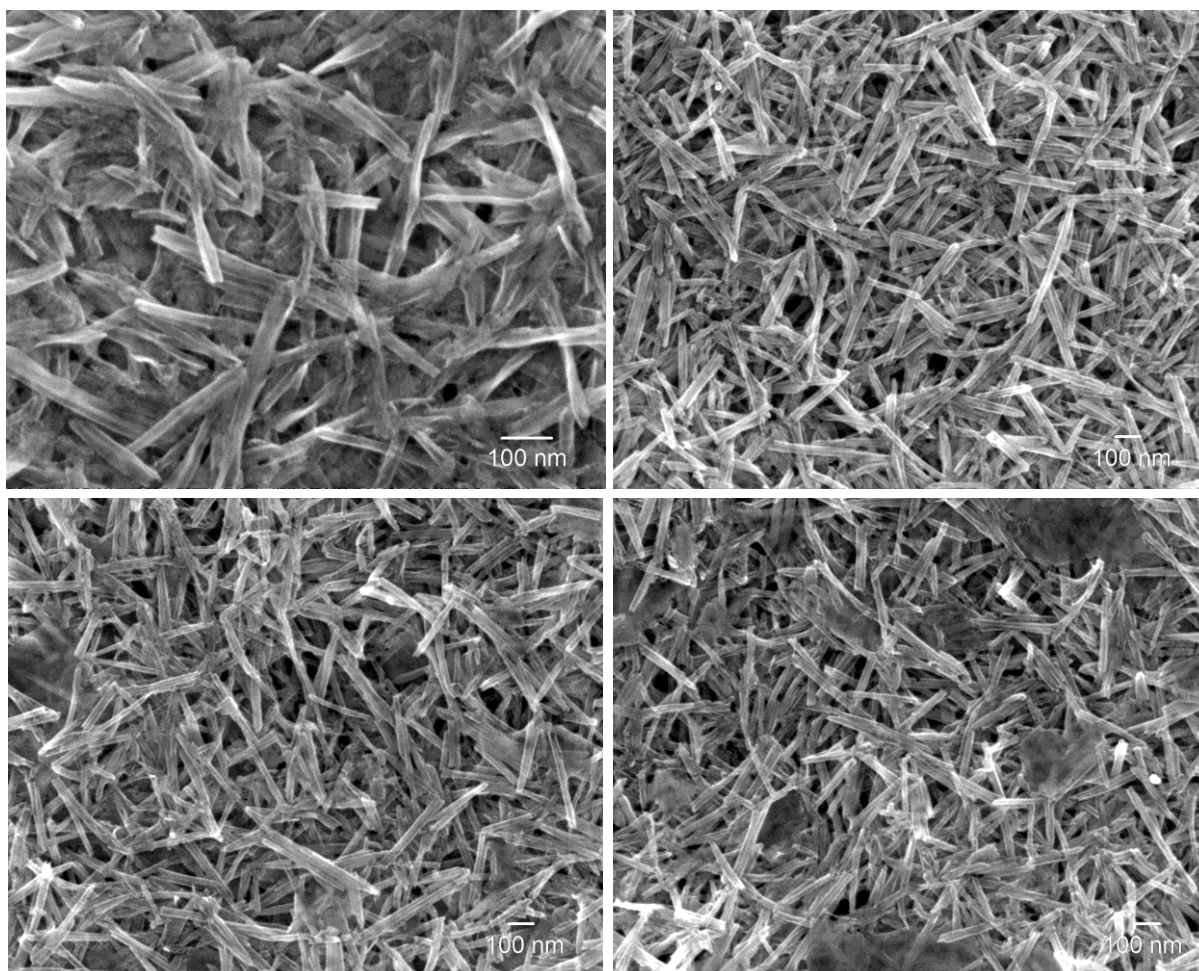
Fig. S1. SEI images of hexaniobate nanoscrolls. These images show the reproducibility of the nanoparticles obtained by exfoliation process.
