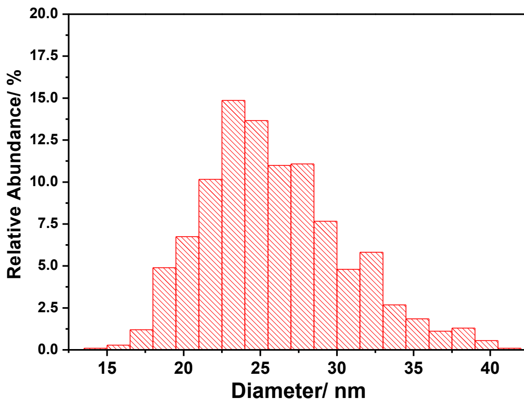
Fig. S2. Histogram of measured external diameters for over one thousand nanoscrolls. The calculated value of the mean external diameter of the NbONsc is 26 \pm 5 nm.
