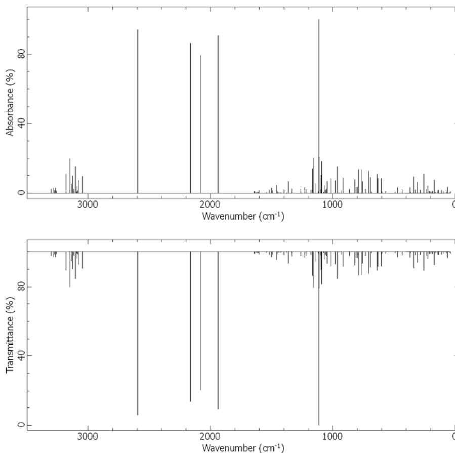
Figure 4. Characteristic infrared spectrum in absorbance and transmittance obtained using the ab initio HF method for the RHF [2-9] in sets of basis RHF/6-311G**(3df, 3pd) [7, 15-21] obtained using computer software GAMESS [15, 20]. Image created by Avogadro software [69, 70].
