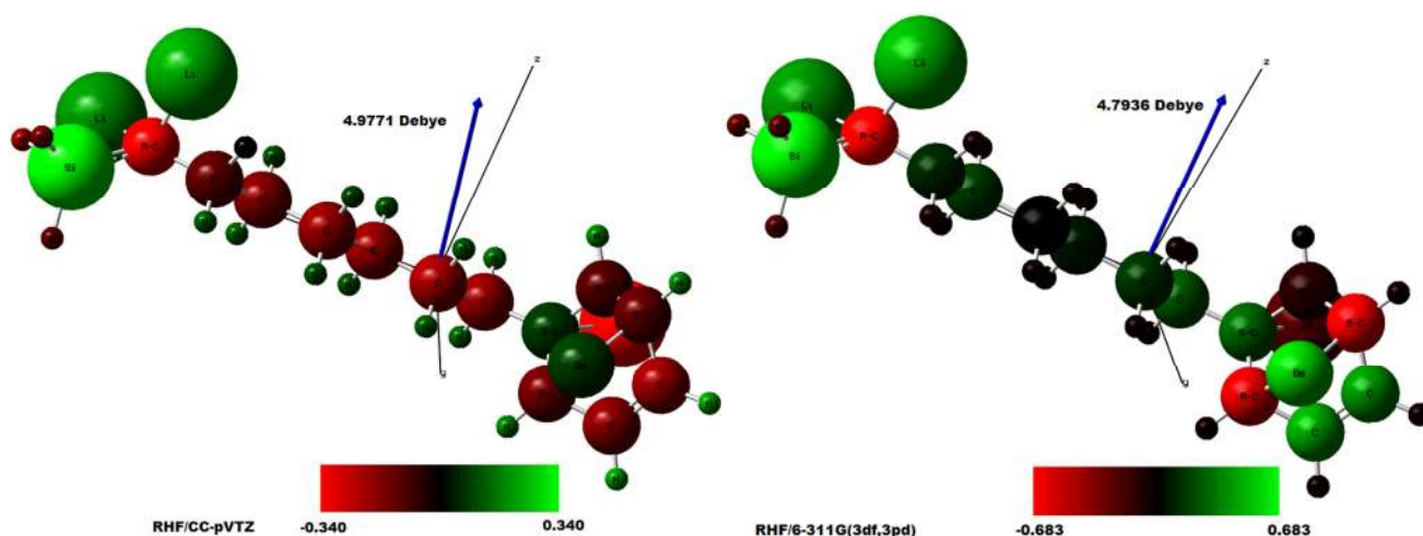
Figure 2. Molecule bio-inorganic C_{13}H_{20}BeLi_2SeSi after dynamics obtained through computer via ab initio calculation method RHF [2-9] in sets of basis obtained using computer software GAMESS [15, 20]. The length of the molecule C_{13}H_{20}BeLi_2SeSi obtained in the base CC-pVTZ [10-14] is of 15.799Å. Represented in green color the positive charge, passing through the absence of color - black - zero charge, for the positive charge red color. A \Delta\delta = 0.680 a.u. of CC-pVTZ [10-14] and \Delta\delta = 1.366 a.u. of 6-311**(3df, 3pd) [7, 15-21], were the elemental charge e ( e = \pm 1,607 \times 10^{-19} C). Images obtained in the software Gaussview, Version 5, 2009 [67].
