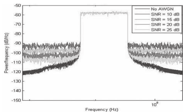
Fig. 13. Spectrum of the GFDM signal before and after passing through the AWGN channel for different SNRs
