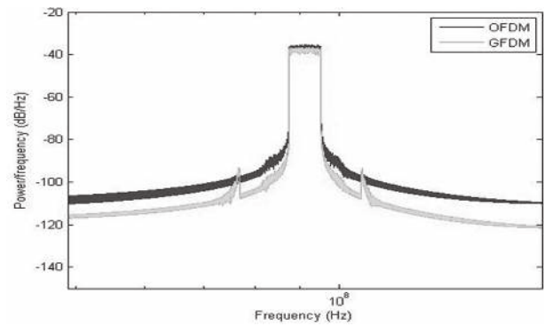
Fig. 12. Spectrum comparison between the GFDM and the OFDM signal
