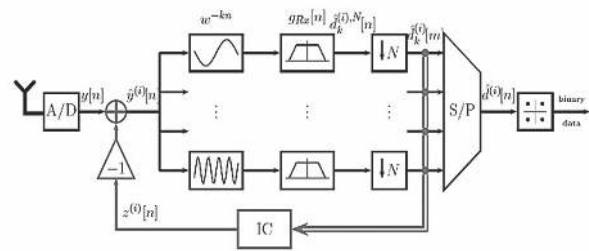
Fig. 2. GFDM matched filter receiver model baseband with interference cancellation [5]
