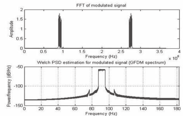
Fig. 10. FFT and GFDm signal spectrum
