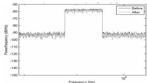
Fig. 14. GFDM signal after passing through the Rayleigh channel
