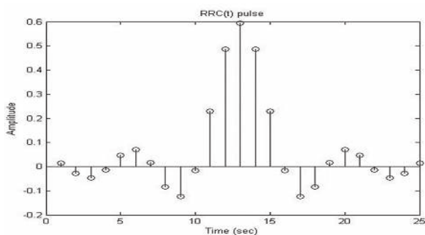
Fig. 5. Impulse response to the root raised cosine pulse
