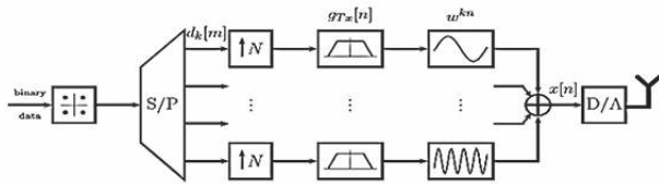
Fig. 1. GFDM baseband transmitter [5]
