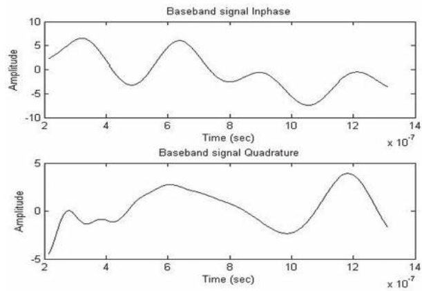
Fig. 8. Baseband signal after filtering
