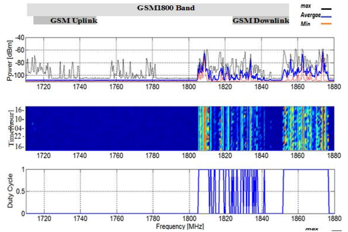
Fig 7. Occupancy measurement from 1710MHz to 1880MHz
