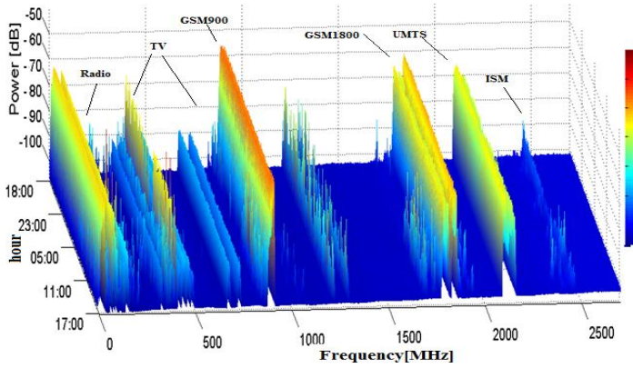
Fig 3. Received power versus the frequency band (80MHz-2700MHz) for 24 hours Start time 10/29/2012 18:00 & Stop time 10/30/2012 18:00
