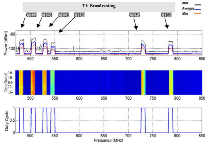
Fig 5. Occupancy measurement from 470MHz to 850MHz
