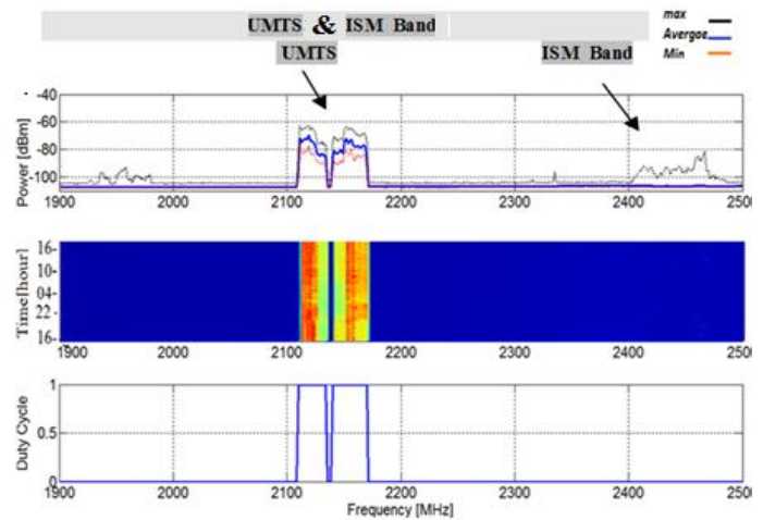
Fig 8. Occupancy measurement from 1900MHz to 2500MHz
