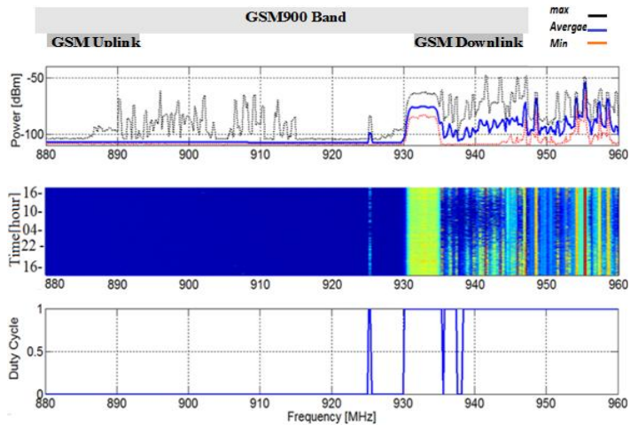
Fig 6. Occupancy measurement from 880MHz to 960MHz
