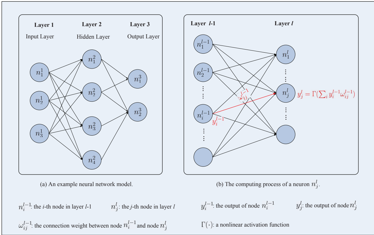
Fig. 4. Multilayer Perceptron Neural Networks
