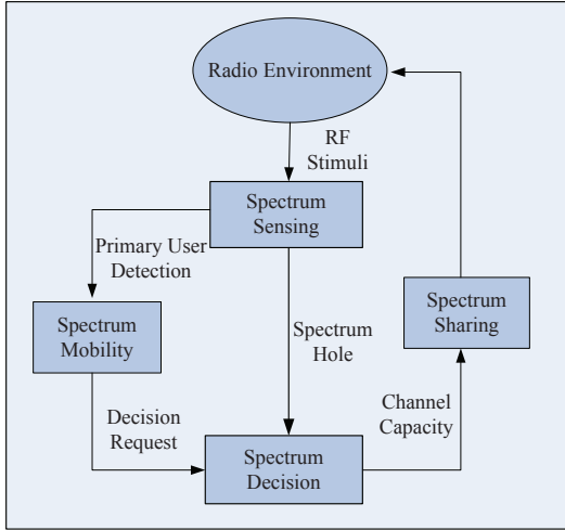
Fig. 2. Operation of the cognitive radio functions
