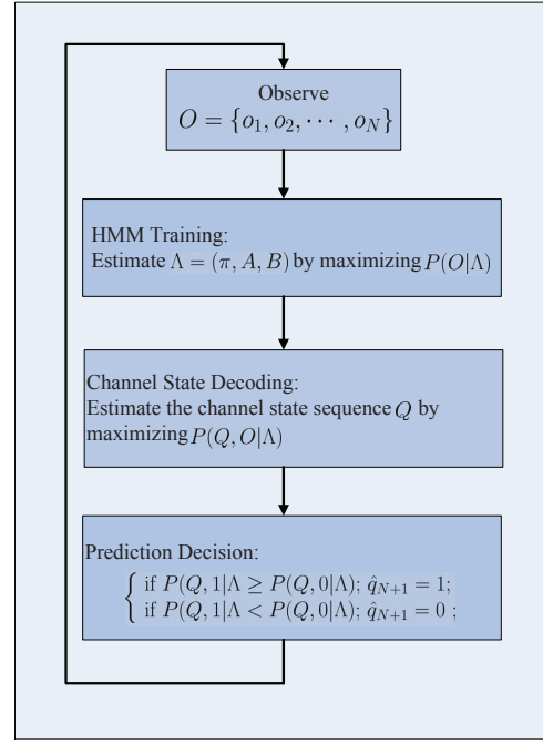
Fig. 3. HMM based prediction
