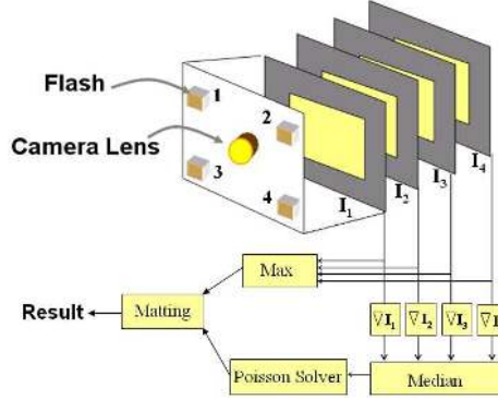
Figure 2: The basic idea of our algorithm for specular reflection reduction.
