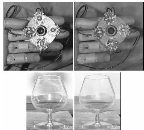
Figure 6. More demonstrations of our method. Left: image taken with one of the flashes. Right: our specular-reduced image.
