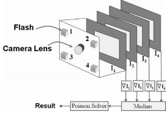
Figure 2. The basic idea of our algorithm for specular reflection reduction.
