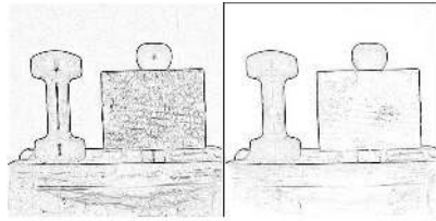
Figure 7. Comparison of depth edge detection without specular reflection reduction (left) and using our method (right).
