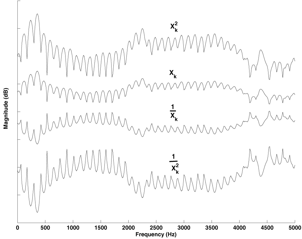
Fig. 1. Plot of the magnitude spectrum, X_k , of a 30-ms segment of the vowel /iy/ taken from the word “heed” (F1 = 344 Hz, F2 = 2450 Hz). Plots of the spectra X_k^2 , 1/X_k and 1/X_k^2 are superimposed for comparison. The latter spectra are shifted relative to X_k for better visual clarity.
