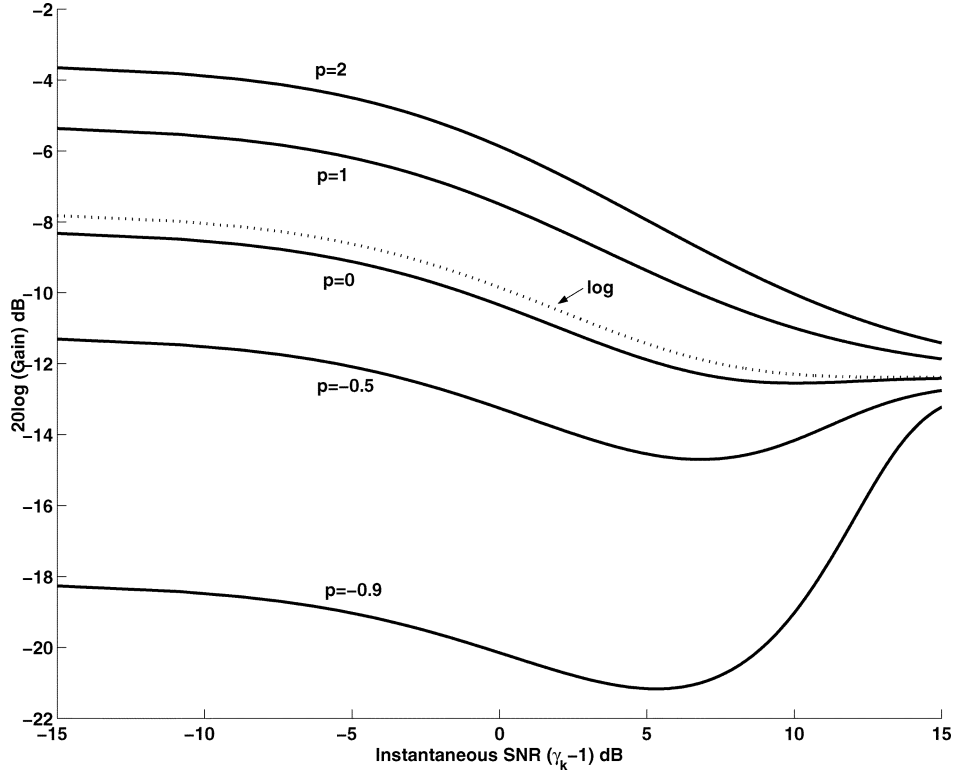
Fig. 4. Gain function of the weighted-cosh estimator [(34)] as a function of the instantaneous SNR (\gamma_k - 1) and for several values of the power exponent p . The a priori SNR is fixed at \xi_k = -5 dB. The gain function of the log-MMSE estimator is also plotted for comparison.
