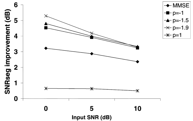
Fig. 6. Performance, in terms of segmental SNR improvement (dB), of the weighted Euclidean estimator [(18)] for different values of p and for different input SNR levels. The performance of the MMSE estimator is also shown for comparison.
