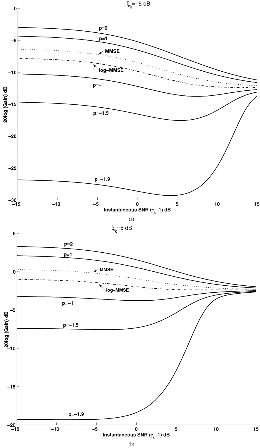
Fig. 2. Gain functions of the weighted-Euclidean distance estimator [(18)] as a function of the instantaneous SNR ( \gamma_k - 1 ) and for several values of the power exponent p . Top panel plots the gain functions for \xi_k = -5 dB and bottom panel plots the gain function for \xi_k = 5 dB. The gain functions of the MMSE and log-MMSE estimators are also plotted for comparison.
