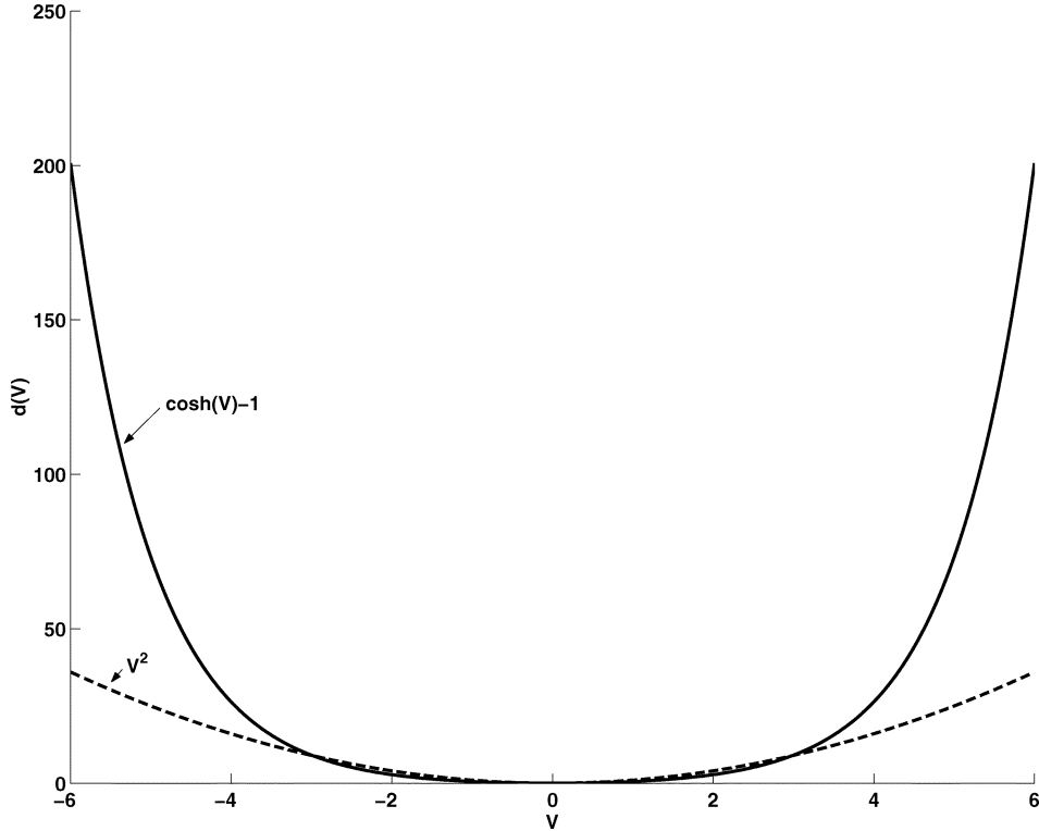
Fig. 3. Plot of the cosh distortion measure d_{\text{cosh}}(V) = \cosh(V) - 1 , where V = \log X_k - \log \hat{X}_k . The log spectral distortion measure [(4)] is also plotted (dashed line) for comparison.
