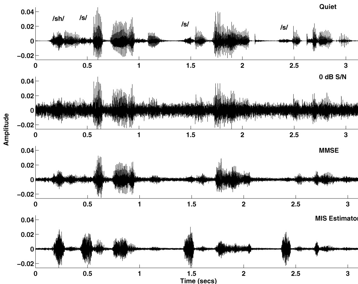
Fig. 8. Top panel shows the waveform of the TIMIT sentence “She was so beautiful, so valiant, so pitiable.” produced by a male speaker. Second panel from the top shows the noisy waveform at 0 dB SNR. The bottom two panels show the enhanced signals by the MMSE and MIS Bayesian estimators. Note that the fricative /s/ at t \approx 0.4, 1.4 and 2.4 secs is hardly present in the signal enhanced by the MMSE estimator, but is quite evident in the signal enhanced by the MIS estimator.
