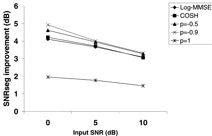
Fig. 7. Performance, in terms of segmental SNR improvement (dB), of the weighted cosh estimator [(34)] for different values of p and for different input SNR levels. The performance of the log-MMSE estimator is also shown for comparison.
