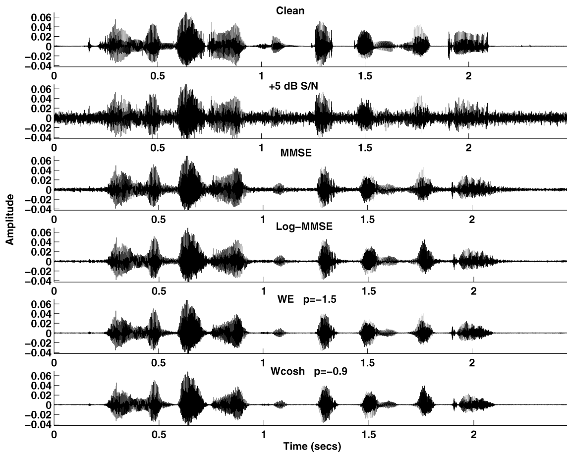
Fig. 9. Top panel shows the waveform of the TIMIT sentence “The angry boy answered, but didn’t look up.” produced by a female speaker. Second panel from the top shows the noisy waveform at 5 dB SNR. The remaining panels show the enhanced signals produced by the MMSE, log-MMSE, weighted-Euclidean estimator ( p = -1.5 ) and weighted-cosh estimator ( p = -0.9 ). Note that the residual noise is significantly reduced by the proposed estimators.
