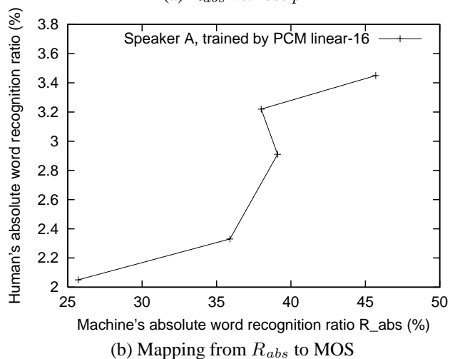
Fig. 5. Importance of voice training using the same codec as test audio clips: irregular results come up if training is by PCM linear-16 instead of G.729
