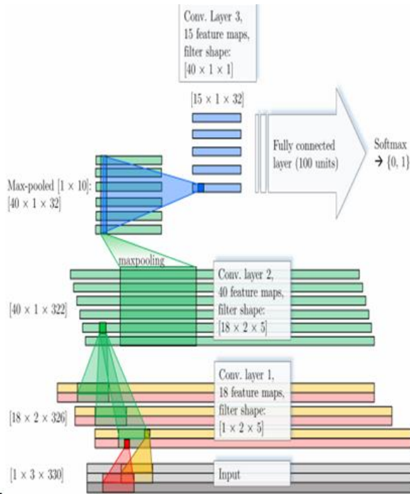
Fig.1: CNN structure
