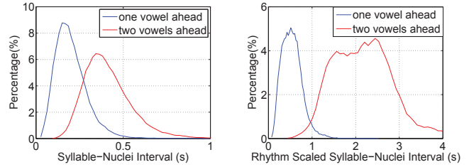
Fig. 3. Distribution of Syllable-Nuclei Intervals in TIMIT and their corresponding rhythm-scaled versions.
