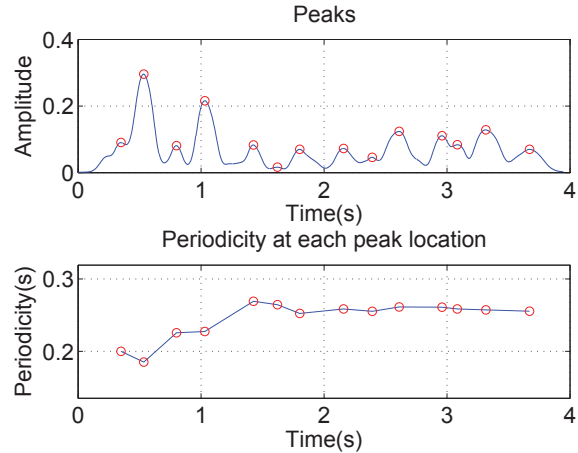
Fig. 4. Example of estimated instantaneous rhythm periodicity for a single TIMIT utterance. See text for details.
