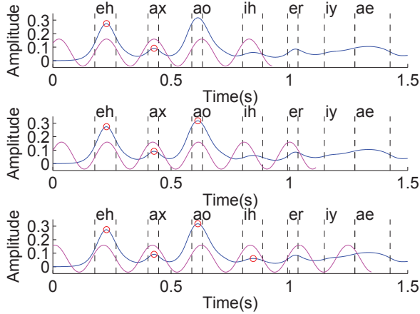
Fig. 2. Example of speech-rhythm based detection of syllable nuclei. See text for details.
