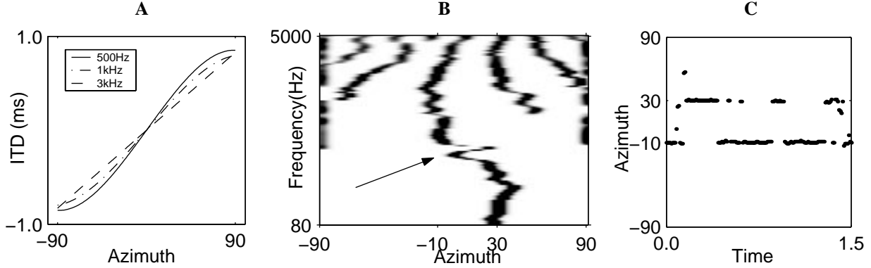
Figure 2. A: Functions relating azimuth to ITD for three channels of the auditory model with CFs of 500Hz, 1kHz, 3kHz. B: Cross-correlation for a mixture of male speech at 30^\circ degrees and female speech at -10^\circ degrees (128 channels, time frame 40 (0.4 ms)). C: Azimuth localization for the two most predominant sources in a mixture of speech at 30^\circ and telephone ringing at -10^\circ updated at every 10 ms.
