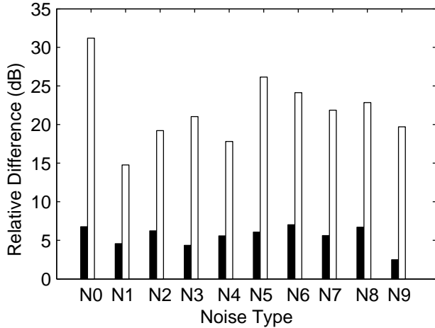
Figure 5: Relative difference from the ideal binary mask using pitch-based algorithm (black bar) and our model (white bar) for voiced speech mixed with ten different types of noise (N0=1kHz tone; N1=random noise; N2=noise burst; N3="cocktail party"; N4=rock music; N5=siren; N6=trill telephone; N7=female speech; N8=male speech; N9=female speech). The voice source is located at 30^\circ and the noise source at -10^\circ .
