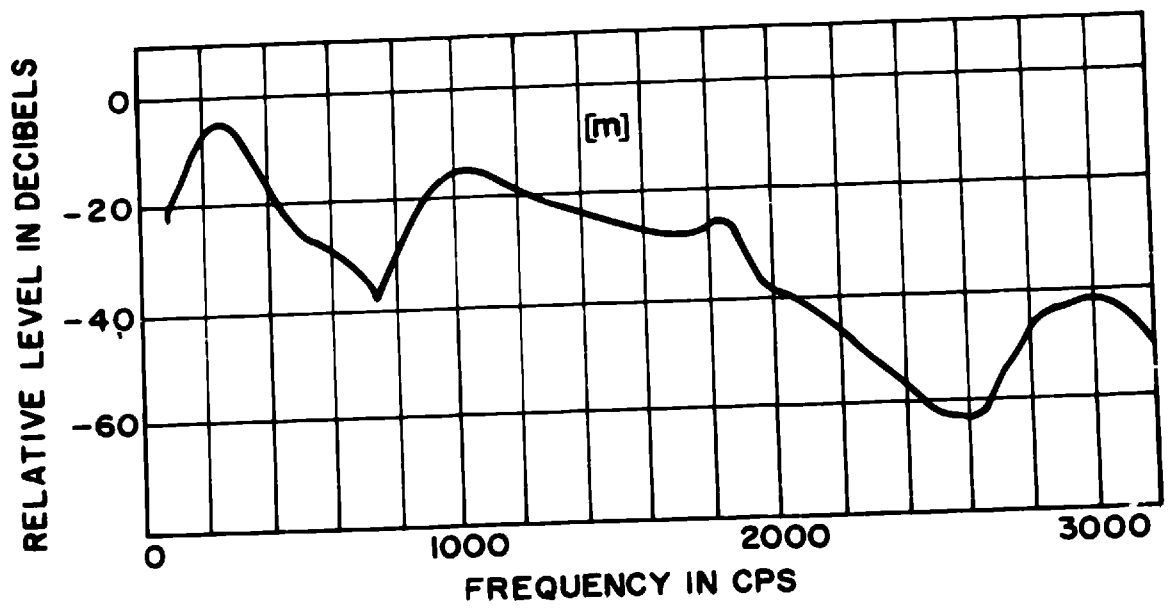
FIGURE 4.4 SPECTRAL ENVELOPE FOR A TYPICAL /m/. ( FROM NAKATA - 1959 )
