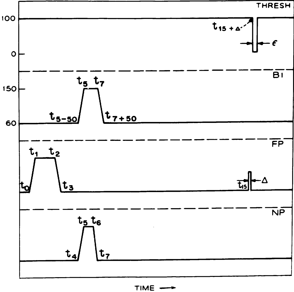
TYPICAL EXAMPLE OF CONTROL PARAMETER CONTOURS FIG. 5.7B
