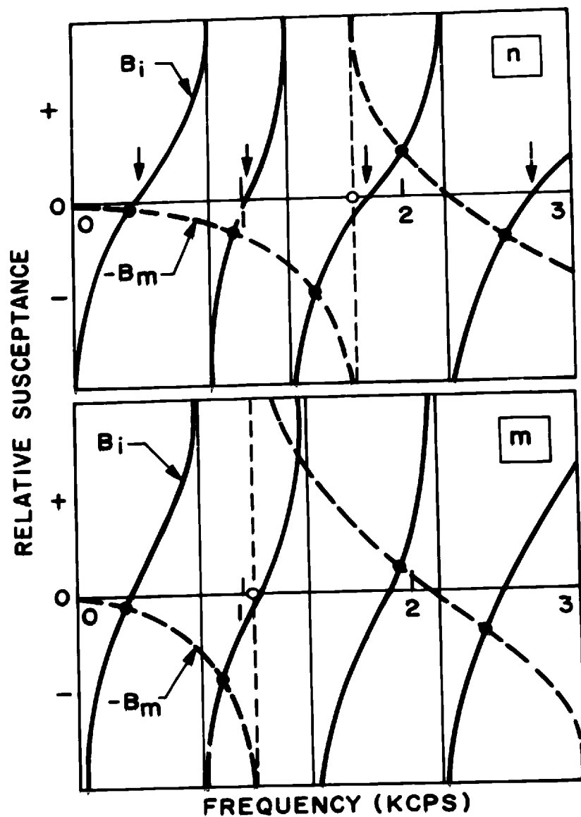
FIGURE 4.3 FREQUENCY CHARACTERISTICS OF SUSCEPTANCES B_i AND B_m (SOLID CIRCLES INDICATE FORMANTS, OPEN CIRCLES INDICATE ANTI-FORMANTS.) (FROM FUJIMURA - 1962)
