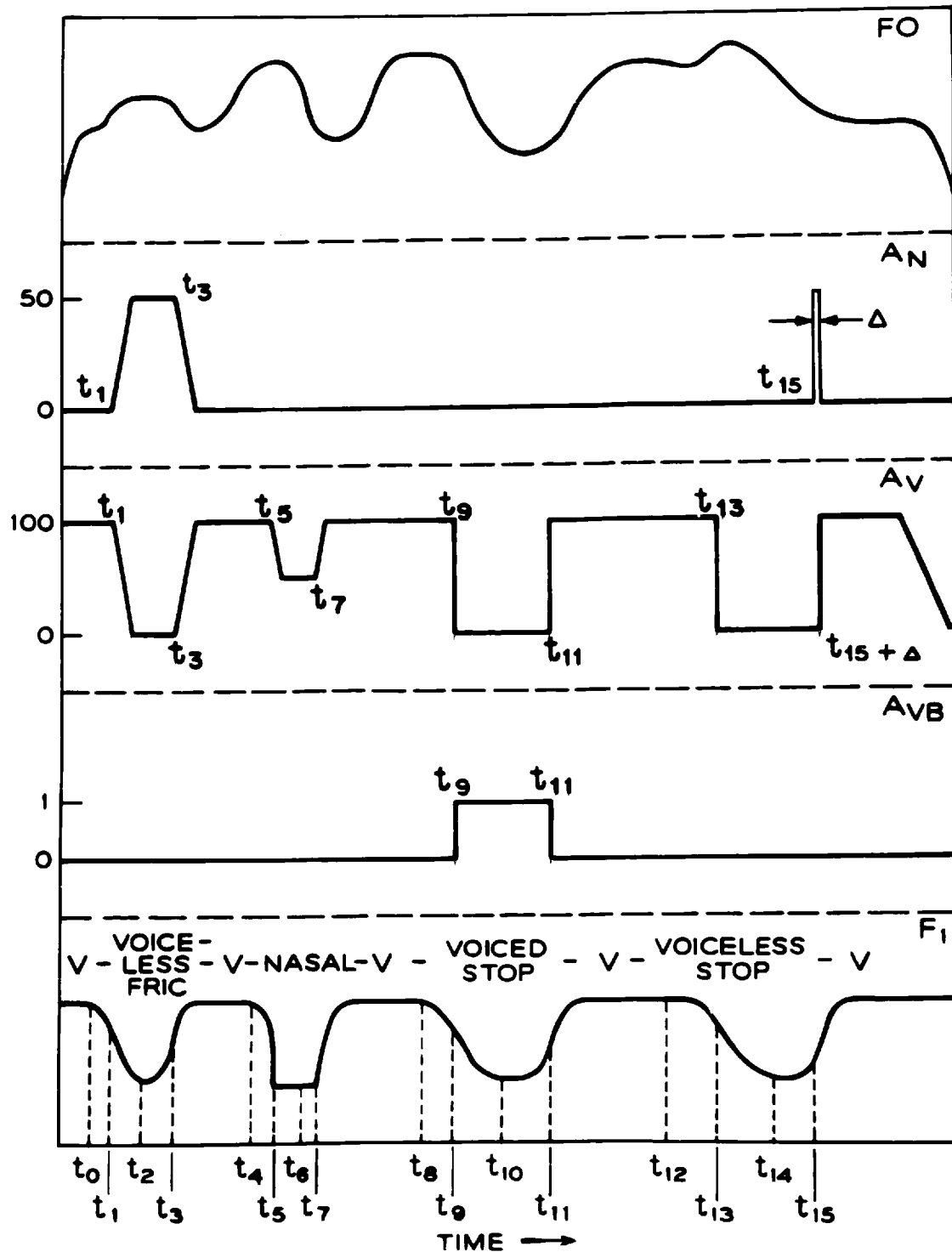
TYPICAL EXAMPLE OF CONTROL PARAMETER CONTOURS FIG. 5.7A
