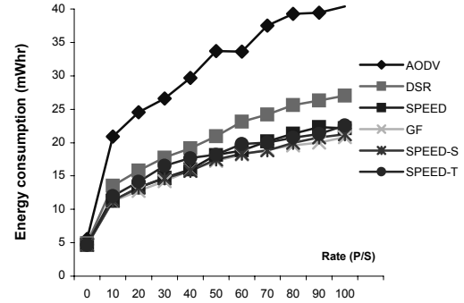
Figure 12. Energy Consumption for transmission
