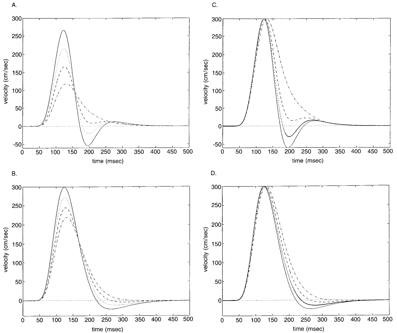
Figure 3. Properties of velocity profiles for movements with different accuracy demands. 3A: Typical velocity profiles corresponding to the quadratic law. — \Delta D/D = 5.71 \cdot 10^{-1} ; .... \Delta D/D = 5.00 \cdot 10^{-1} ; ---- \Delta D/D = 4.00 \cdot 10^{-1} ; - - - \Delta D/D = 2.50 \cdot 10^{-1} . 3B: Typical velocity profiles corresponding to the power law. — \Delta D/D = 5.77 \cdot 10^{-1} ; .... \Delta D/D = 5.05 \cdot 10^{-1} ; ---- \Delta D/D = 3.85 \cdot 10^{-1} ; - - - \Delta D/D = 1.44 \cdot 10^{-1} . (C) and (D) Approximate superimposition of the profiles of 3A and 3B, respectively, after amplitude rescaling.
