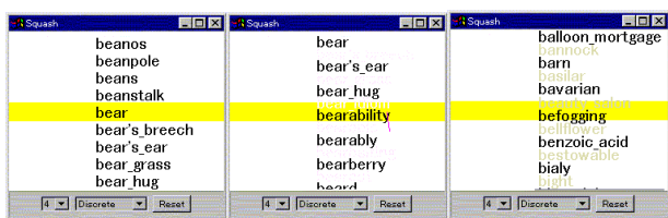
a) static view b) scrolling slowly c) scrolling fast
