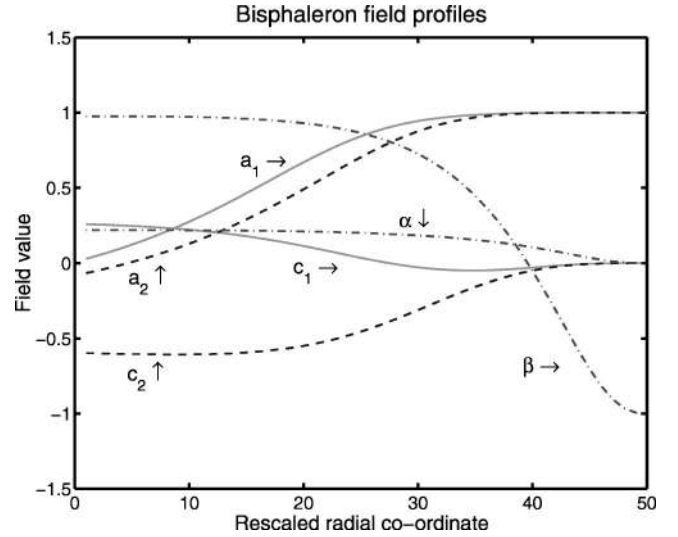
FIG. 18. The bisphaleron field profiles for \tan\beta=6.0 , M_h=15.0M_W , M_H=17.0M_W , M_A=2.0M_W , M_{H^\pm}=3.0M_W and \lambda_3=-0.1 . It has energy= 4.932 M_W/\alpha_W , n_{CS}=0.569 , two negative curvature eigenvalues -11.915M_W^2 , and -6.788M_W^2 . Its conjugate partner is the identical solution under P conjugation ( \alpha \rightarrow -\alpha ), and has n_{CS}=0.431 .
