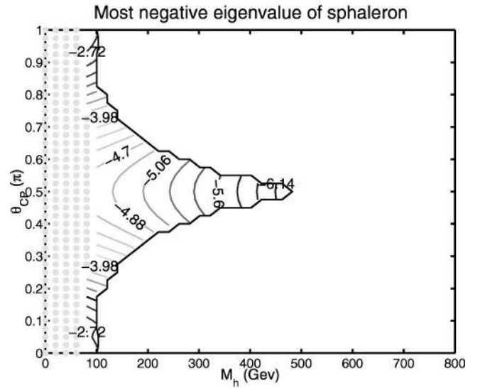
FIG. 12. Top: contours in M_h , \theta_{CP} space of the energy ( M_W/\alpha_W ) of sphaleron; bottom: of the negative eigenvalue of the sphaleron ( M_W^2 ). For this region of parameter space the sphaleron is the only solution. For the blank region Eq. (10) is not the global minimum. For the dotted region the potential is unbounded. The input parameters are \phi=0.125\pi , \psi=0.0 , M_H=110 GeV, M_A=500 GeV, M_{H^\pm}=500 GeV, and \lambda_3=0.0 . \tan\beta=2.4 .
