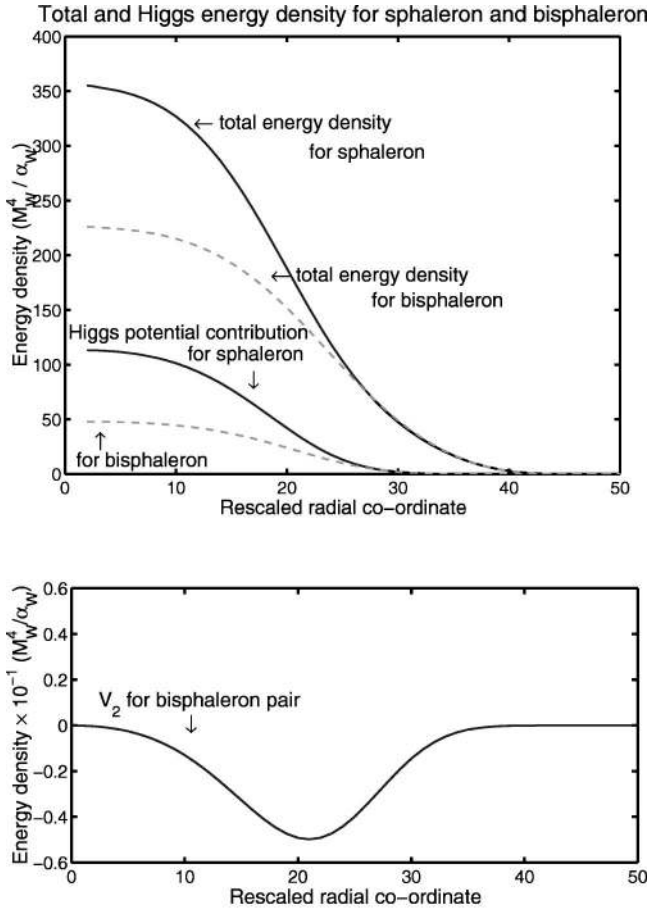
FIG. 17. The top figure shows total and Higgs potential contribution to energy density ( M_W^4/\alpha_W ) for the sphaleron (solid) and the bisphaleron (dashes). The bottom figure shows V_2 for the bisphaleron solution and its conjugate. V_2 for both the bisphaleron and conjugate solution are equal. Input parameters are \tan\beta=6.0 , \theta_{CP}=0.0 , \phi=0.0 , \psi=0.0 , M_h=15.0M_W , M_H=17.0M_W , M_A=2.0M_W , M_{H^\pm}=3.0M_W , and \lambda_3=-0.1 .
