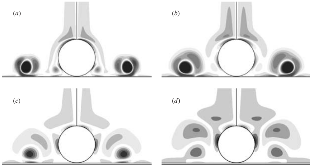
FIGURE 11. Vorticity contours showing the long-time-evolution vortex structures for Re = 1500 . (a) \tau = 8 , (b) \tau = 16 , (c) \tau = 32 , (d) \tau = 52 . For each image the contour levels have been adjusted to show all the vortex structures present. Note the net movement of the primary vortex ring back towards the axis.
