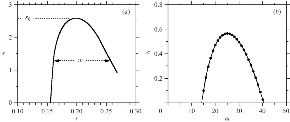
FIGURE 26. (a) Local inviscid growth rate s = (-\Phi)^{1/2} and (b) global viscous growth rate as functions of the azimuthal wave number m , for the flow field in figures 25 b and 25 c , according to (4.4).
