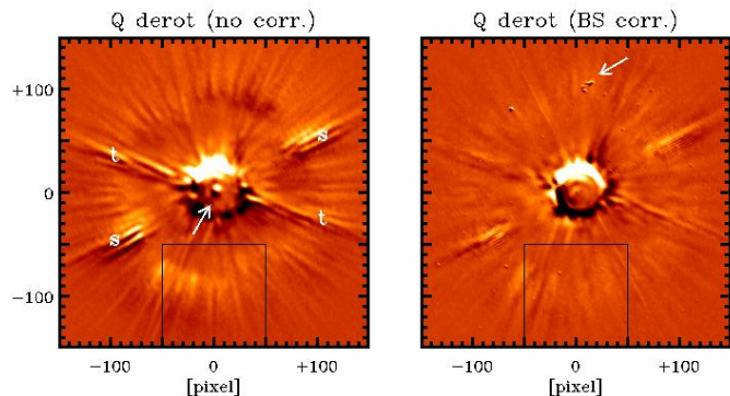
Fig. 28. Beam shift effect for \alpha Cen B in the VBB filter for a coronagraphic (CLC-MT-WF) Stokes Q frame ( left ) and the beam shift corrected frame ( right ) for essentially the same instrument configuration as the stellar PSF in Fig. 26. The arrow in the left panel points to the PSF peak transmitted through the mask. PSF residual features are marked in the left panel with “t” and “s” according to Fig. 8. In the right panel the arrow points to one of several spots from the camera, which show up because of the applied beam-shift correction. The squares at the bottom mark the area for the reported \sigma(Q) .
