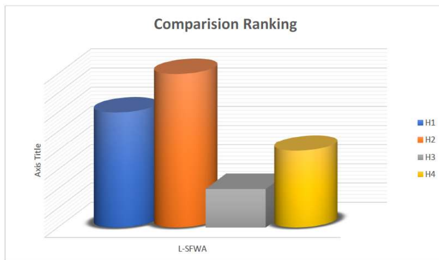
Figure 6. Comparison Ranking.
