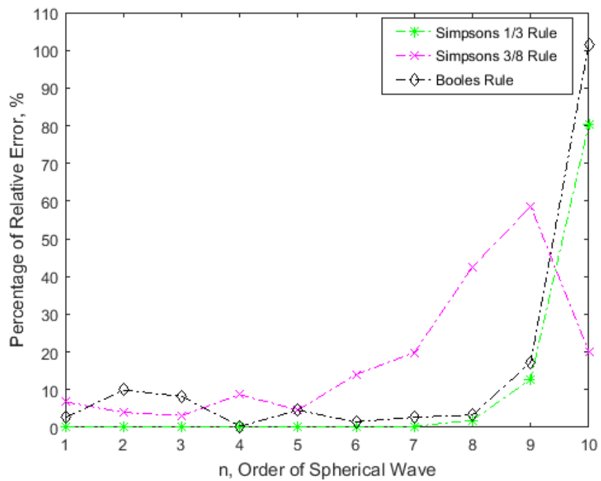
Figure 5.5 Comparison of Simpson's 1/3, 3/8 and Boole's Rule for 21 Sample Points
