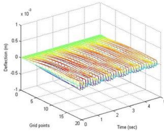
Fig.11. Fluctuation of beam along the length following the cancellation with the implementation of AVC using SNN
