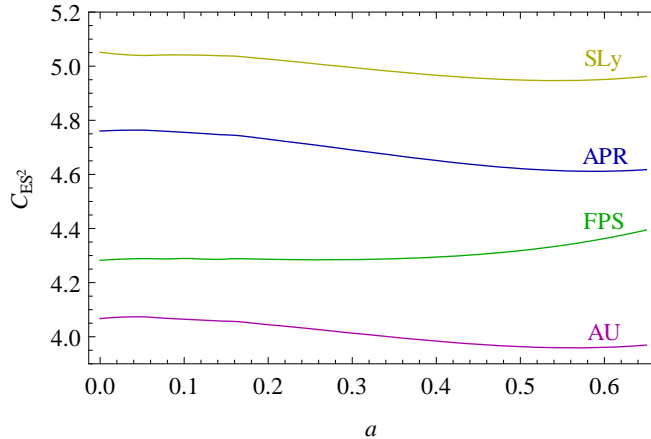
Figure 1: The coefficient C_{ES^2} as a function of the dimensionless spin a = S/G\mu^2 , where \mu is identified with the gravitating mass and is given by \mu = 1.4M_\odot here. The data points were generated using the RNS code [42, 43], where a multipole extraction according to [49] was used. The labels SLy, APR, FPS, and AU refer to equations of state considered in [50].
