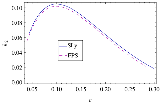
Figure 4: Dimensionless quadrupolar Love number k_2 as a function of the compactness c = R_S/2R for two different equations of state (SLy, FPS).
