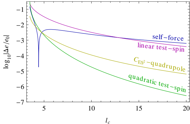
Figure 2: Various corrections to the binding energy e for a maximally spinning (small) black hole in a Schwarzschild background. Here l_c := J_\phi - S is the orbital angular momentum. The mass ratio is formally taken to be q = 1 in the plot, though the result are only valid for q \ll 1 . The curves can be scaled to the case of interest ( q \lesssim 10^{-2} ): self-force and linear spin effects scale as \propto q , the others as \propto q^2 .
