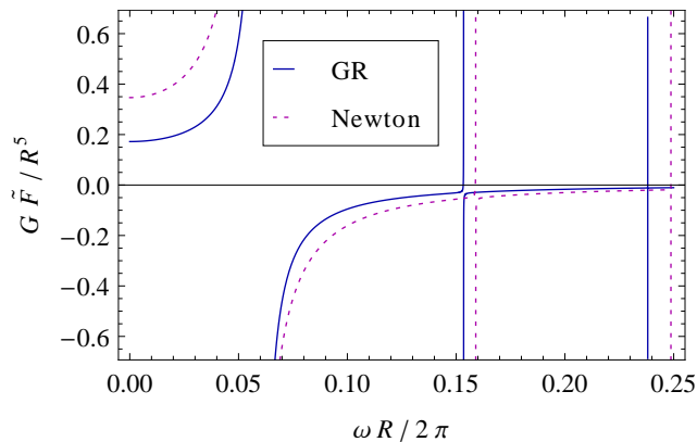
Figure 3: Response function of the quadrupole, l = 2 , for a one solar mass star. The equation of state is a polytrope with index 1 and such that the radius R is 17.7 km in the Newtonian case or 15.7 km in the relativistic case.
